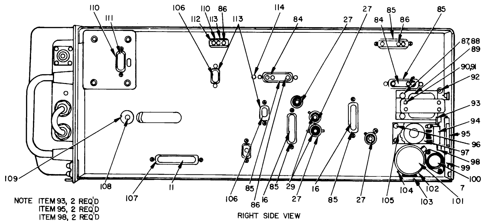
Figure 3. Chassis Assembly (Sheet 2 of 2).
