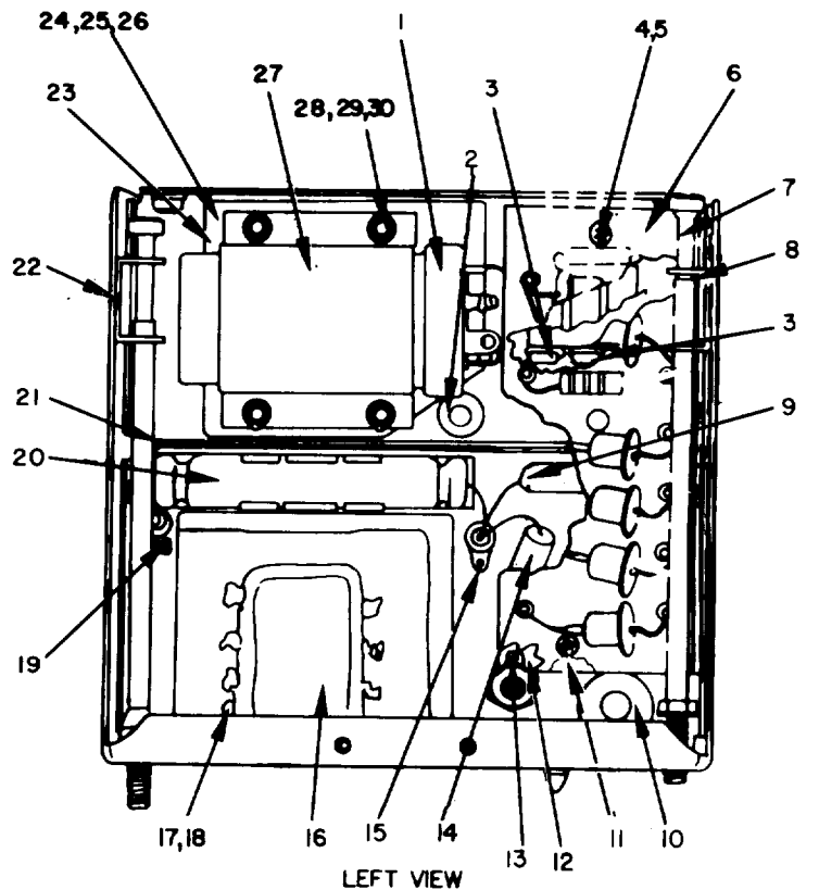
LEFT VIEW
