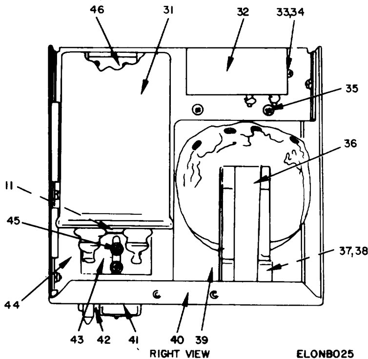
RIGHT VIEW
