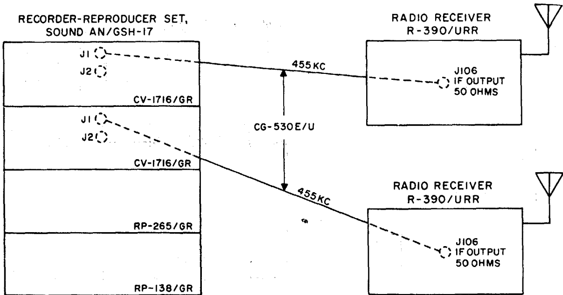
Figure 2-7. Setup for receiving coder-burst transmission for a permission equipment check.
