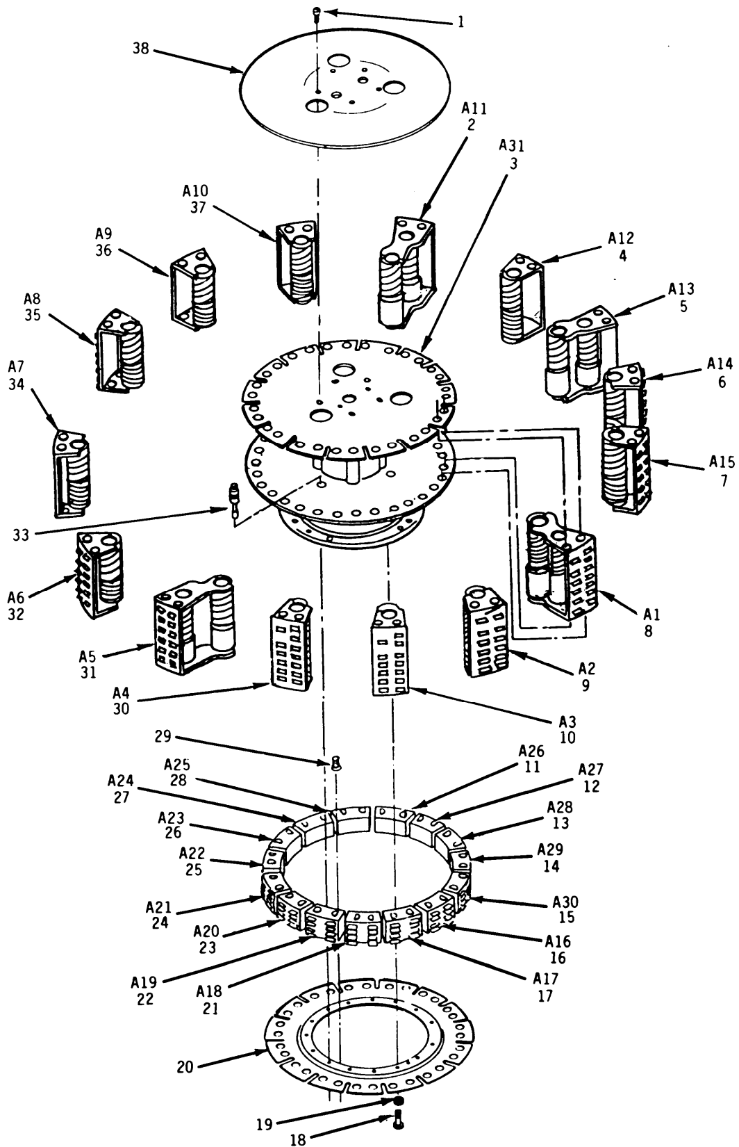
FIGURE 41. Drum, Turret 2A2A1
