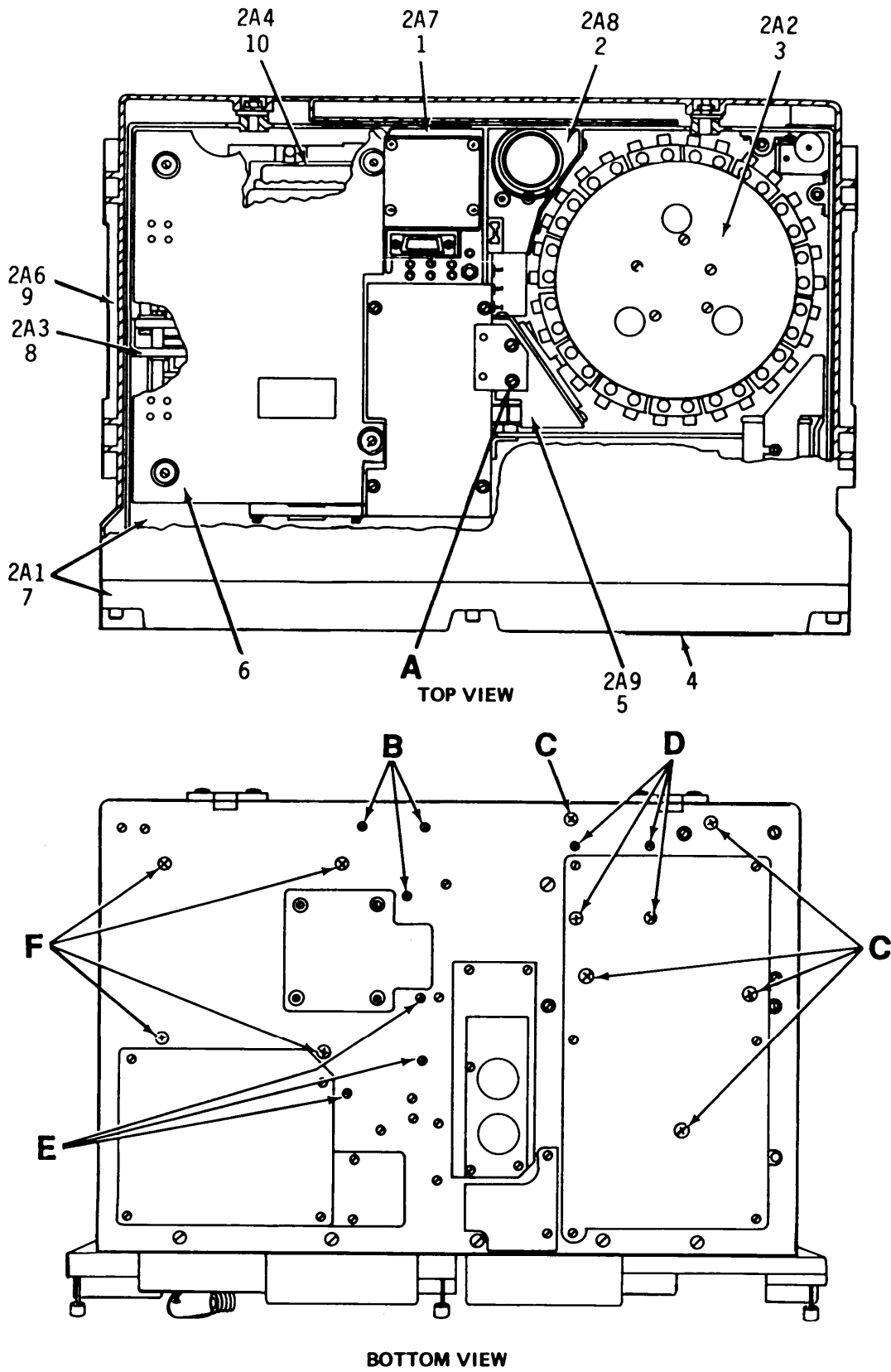
FIGURE 23. Amplifier, Radio Frequency AM-3349/GRC-106 (Sheet 1 of 2)
