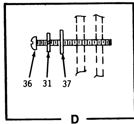
FIGURE 6. Chassis Assembly 1A1A2 (Sheet 3 of 3)
