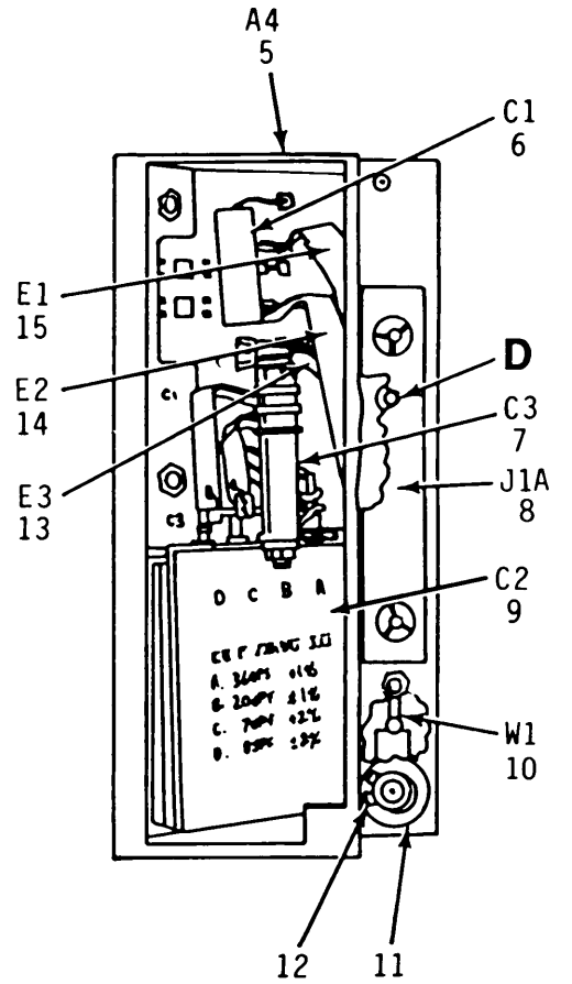
REAR VIEW
