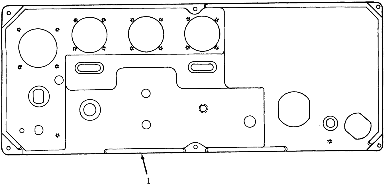
FRONT SIDE VIEW
