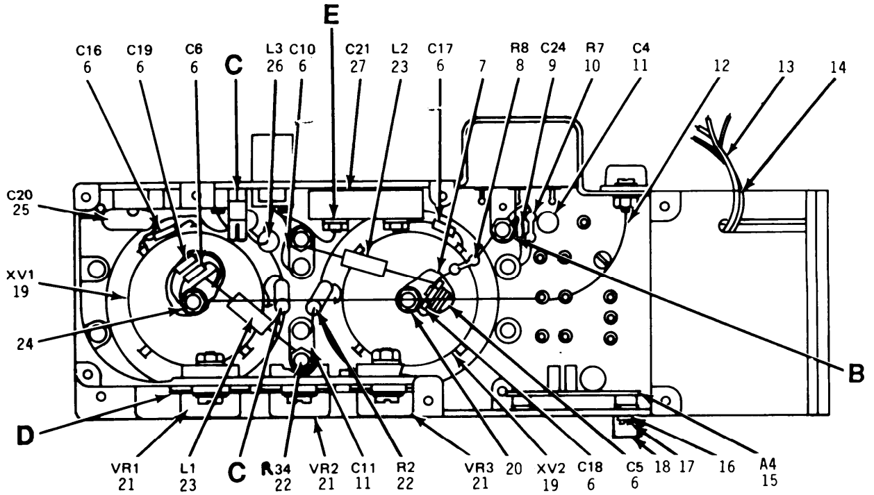
TOP INTERIOR VIEW
