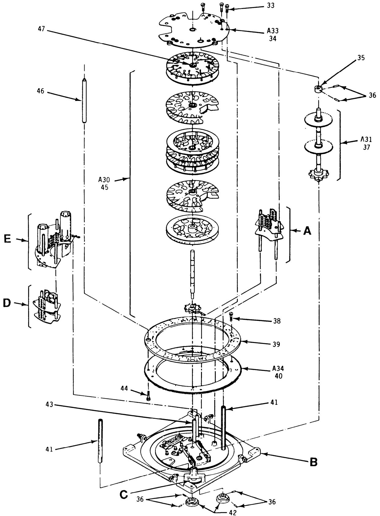
NOTE: FOR COMPLETE REFERENCE DESIGNATION PREFIX WITH 1A12. FIGURE 21. RF Amplifier Module 1A12 (Sheet 2 of 7)
