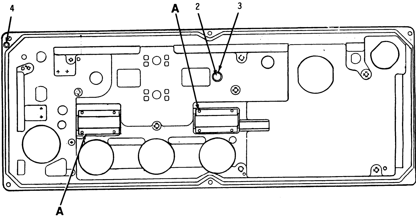
REAR SIDE VIEW
