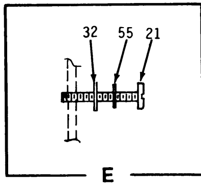
FIGURE 25. Chassis Assembly 2A1A1 (Sheet 4 of 4)
