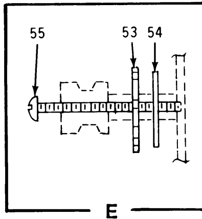
FIGURE 4. Front Panel Assembly 1A1A1 (Sheet 3 of 5)
