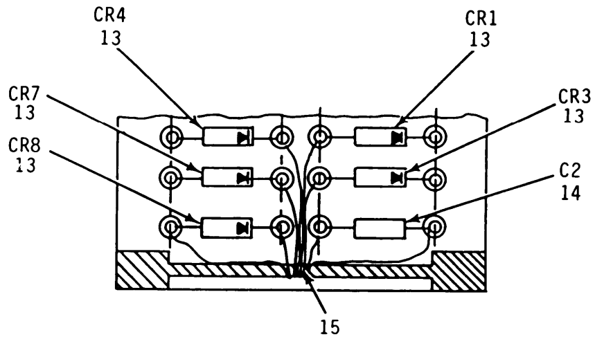
PARTIAL RIGHT INSIDE VIEW
