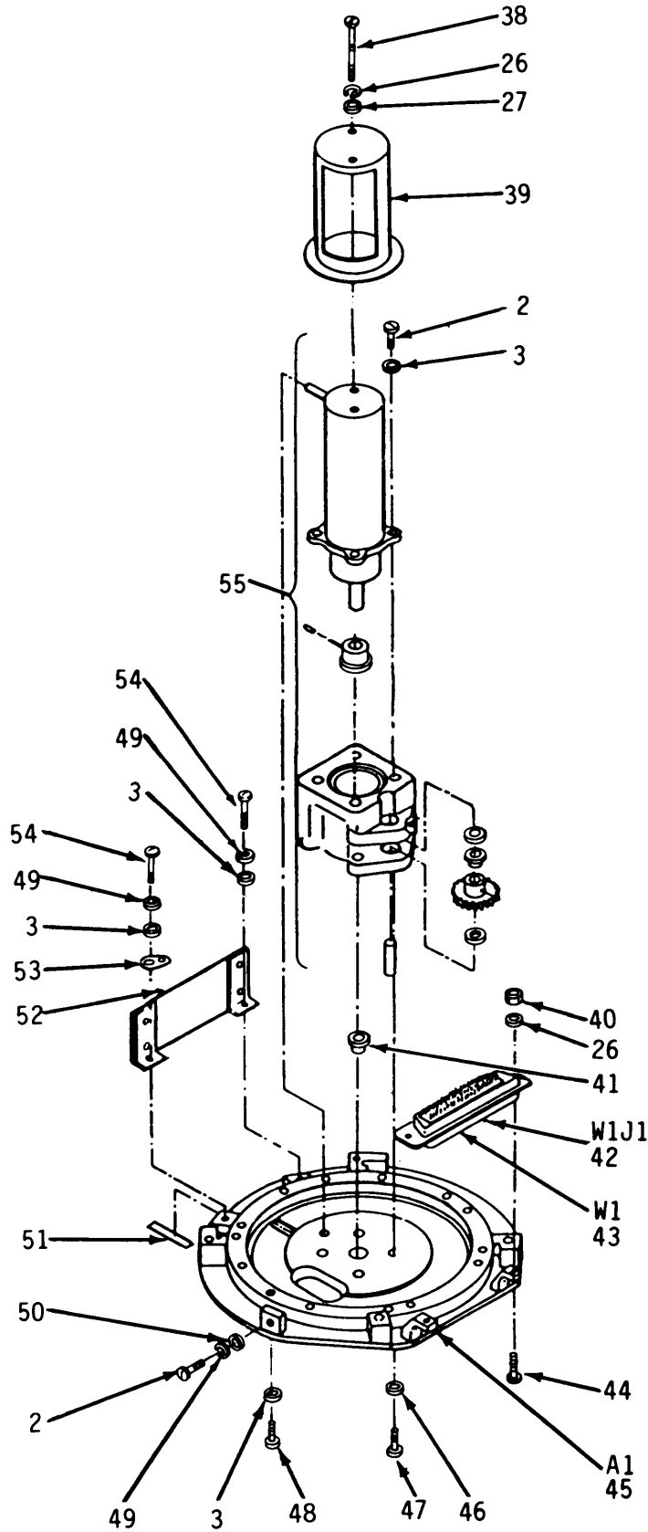
FIGURE 42. Drive, Turret 2A2A2 (Sheet 4 of 4)
