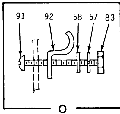
FIGURE 4. Front Panel Assembly 1A1A1 (Sheet 5 of 5)
