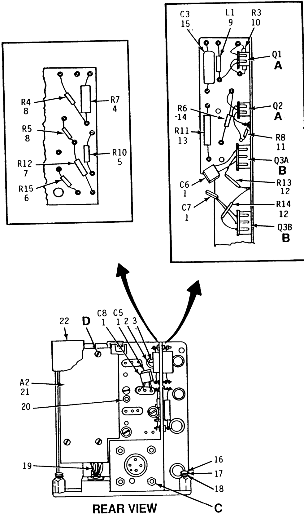
FIGURE 19. Receiver Audio Module 1A10 (Sheet 1 of 3)
