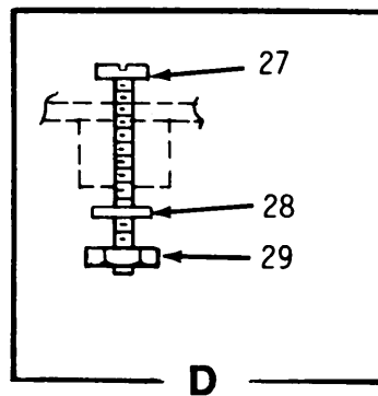
FIGURE 46. Inverter Assembly 2A6A1 (Sheet 2 of 2)
