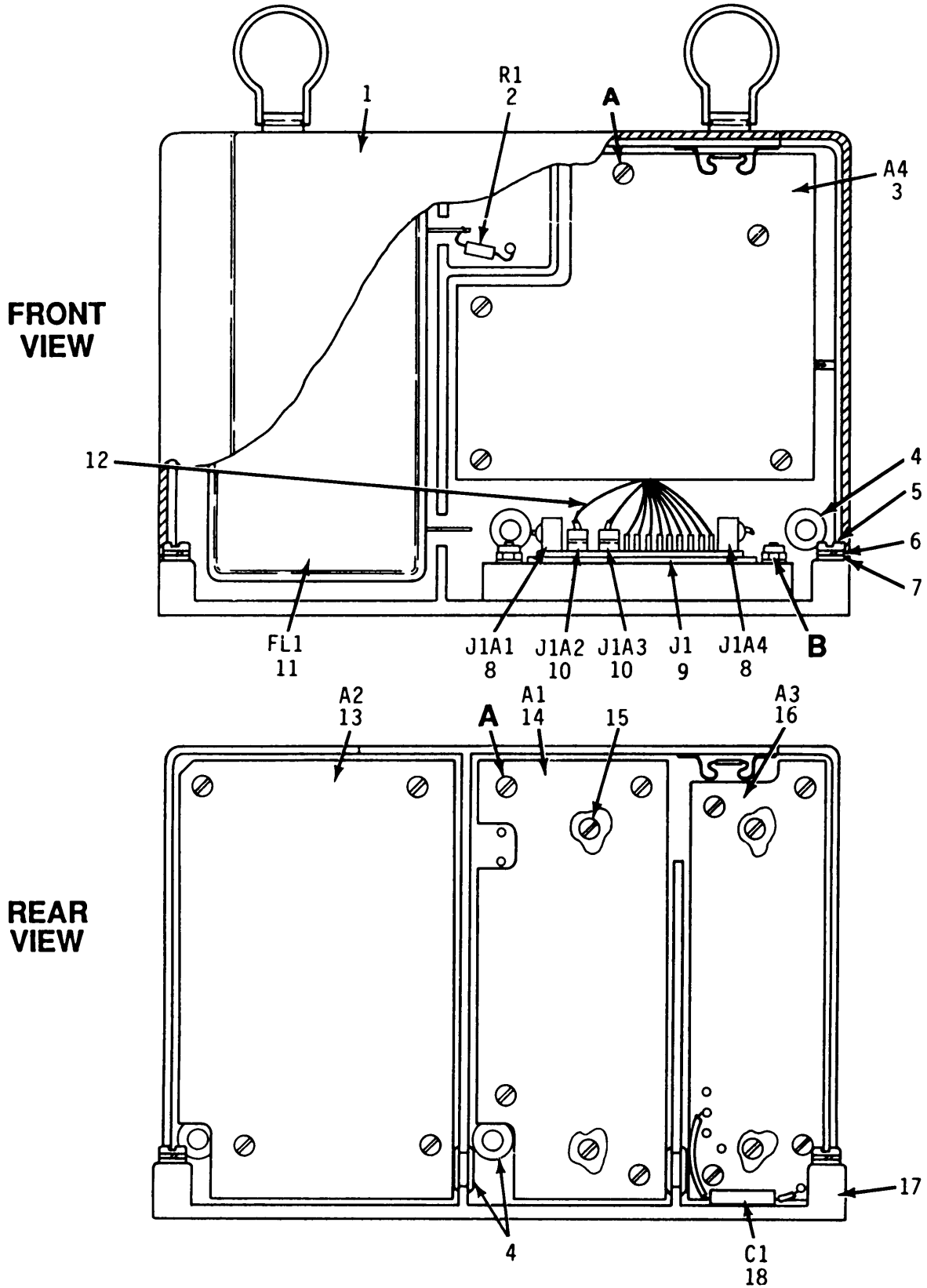
FIGURE 16. Receiver IF Module 1A7 (Sheet 1 of 2)
