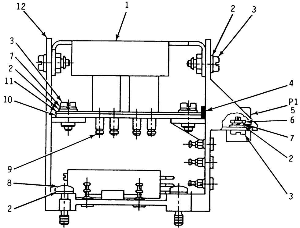
FRONT VIEW
