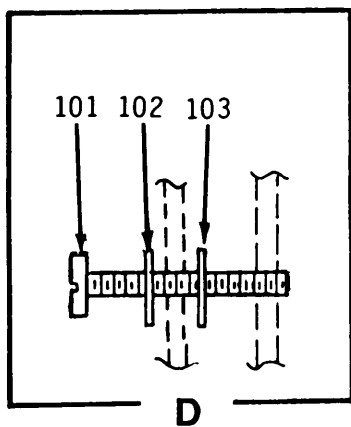
FIGURE 30. Power Amplifier Panel 2A1A5 (Sheet 6 of 6)
