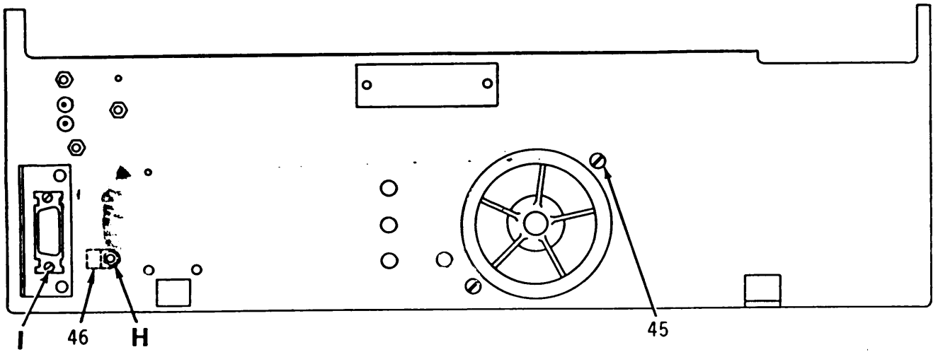
REAR VIEW
