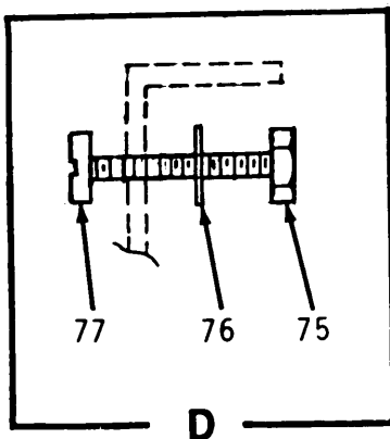
FIGURE 3. Panel-Chassis Assembly 1A1 (Sheet 5 of 5)
