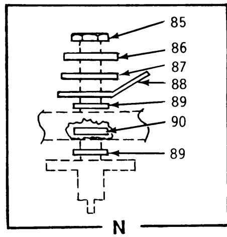
FIGURE 4. Front Panel Assembly 1A1A1 (Sheet 5 of 5)
