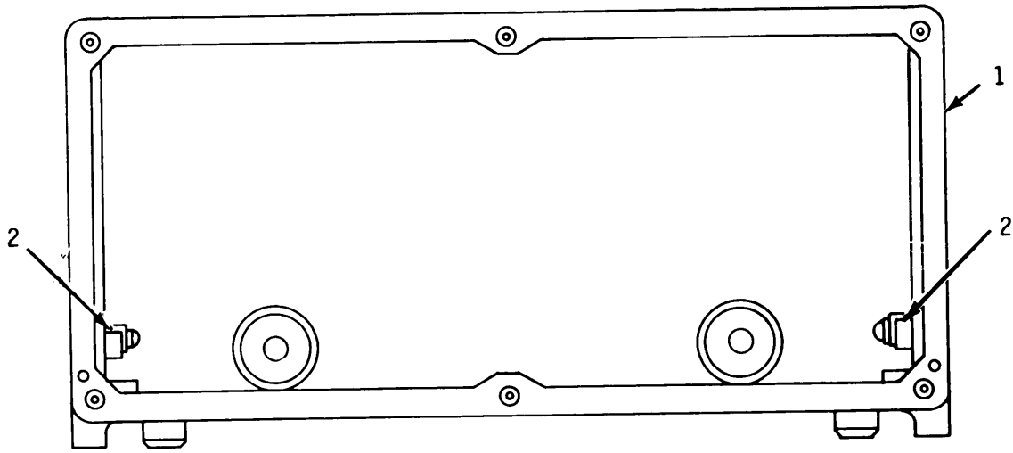
REAR INSIDE VIEW
