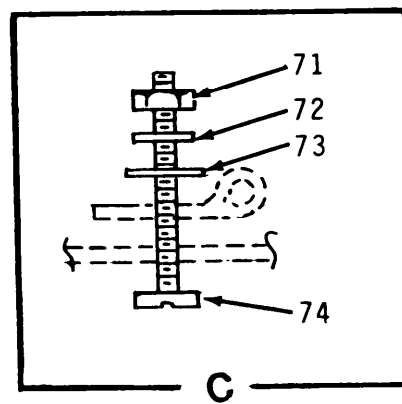
FIGURE 3. Panel-Chassis Assembly 1A1 (Sheet 5 of 5)
