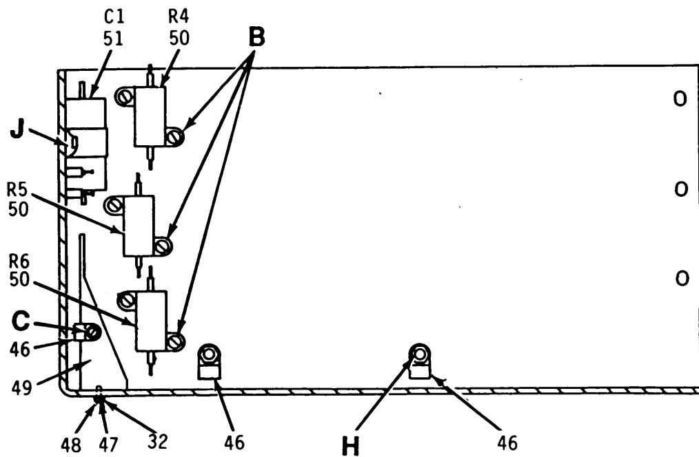
INSIDE REAR VIEW
