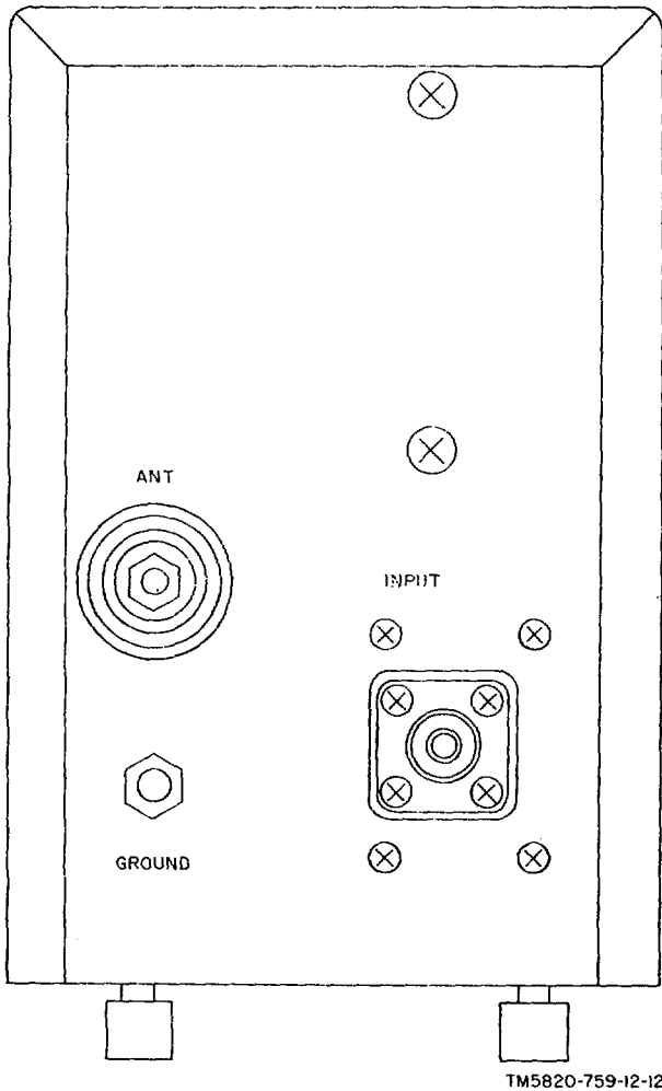
Figure 3-4. Coupler, Antenna CU-17821/ GRC-165, rear panel.
