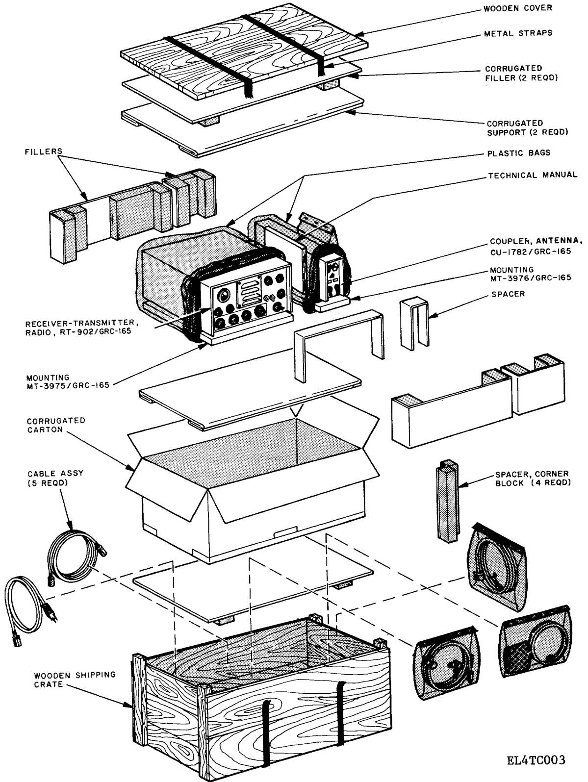
Figure 2-1. Typical packaging.
