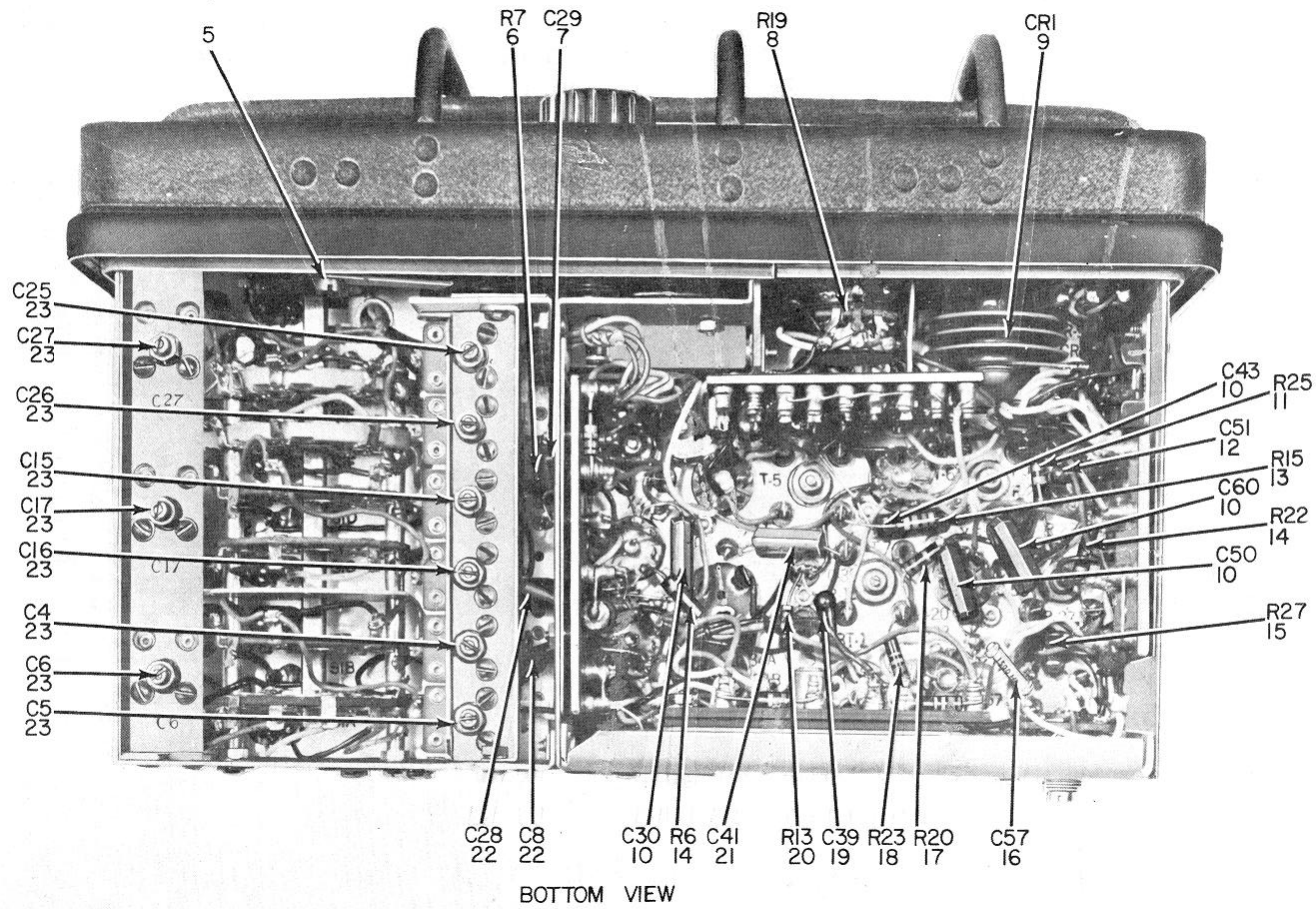
Figure 5.② Receiver-Transmitter RT-77/GRC (Sheet 2 of 6).
