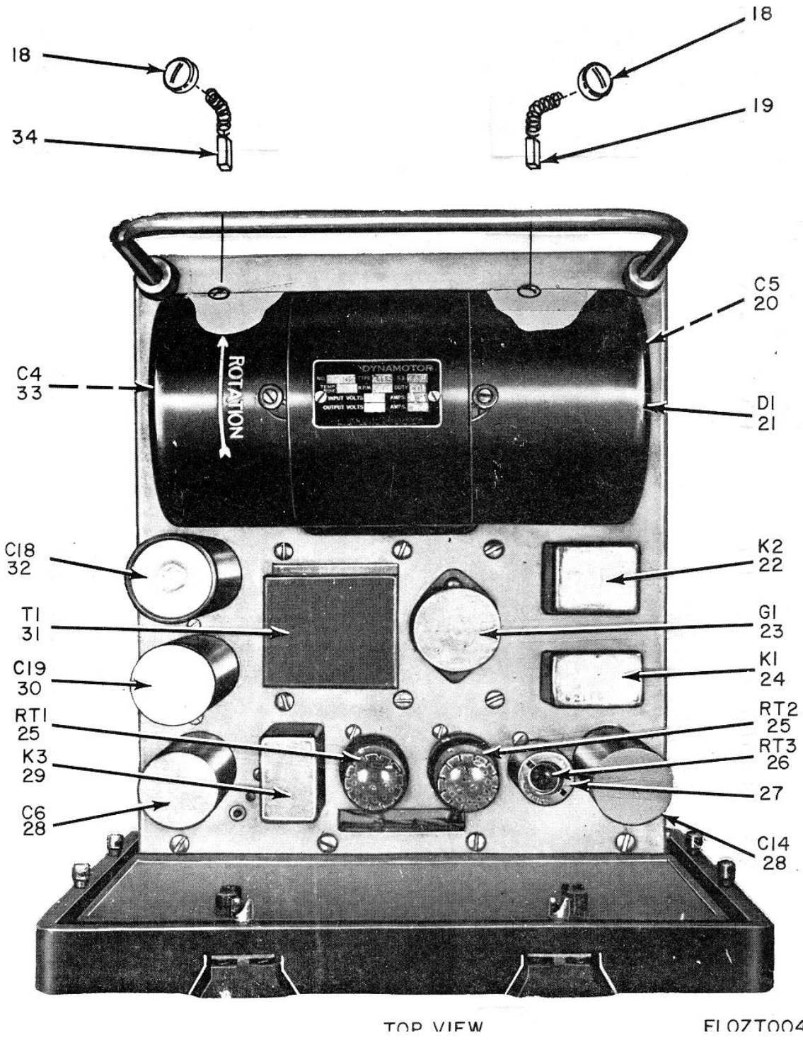
Figure 3.② Dynamotor-Power Supplies DY-88/GRC-9, DY-105/GRC-9X, DY-105A/GRC-9X, DY-105B/GRC-9X, (Sheet 2 of 3).
