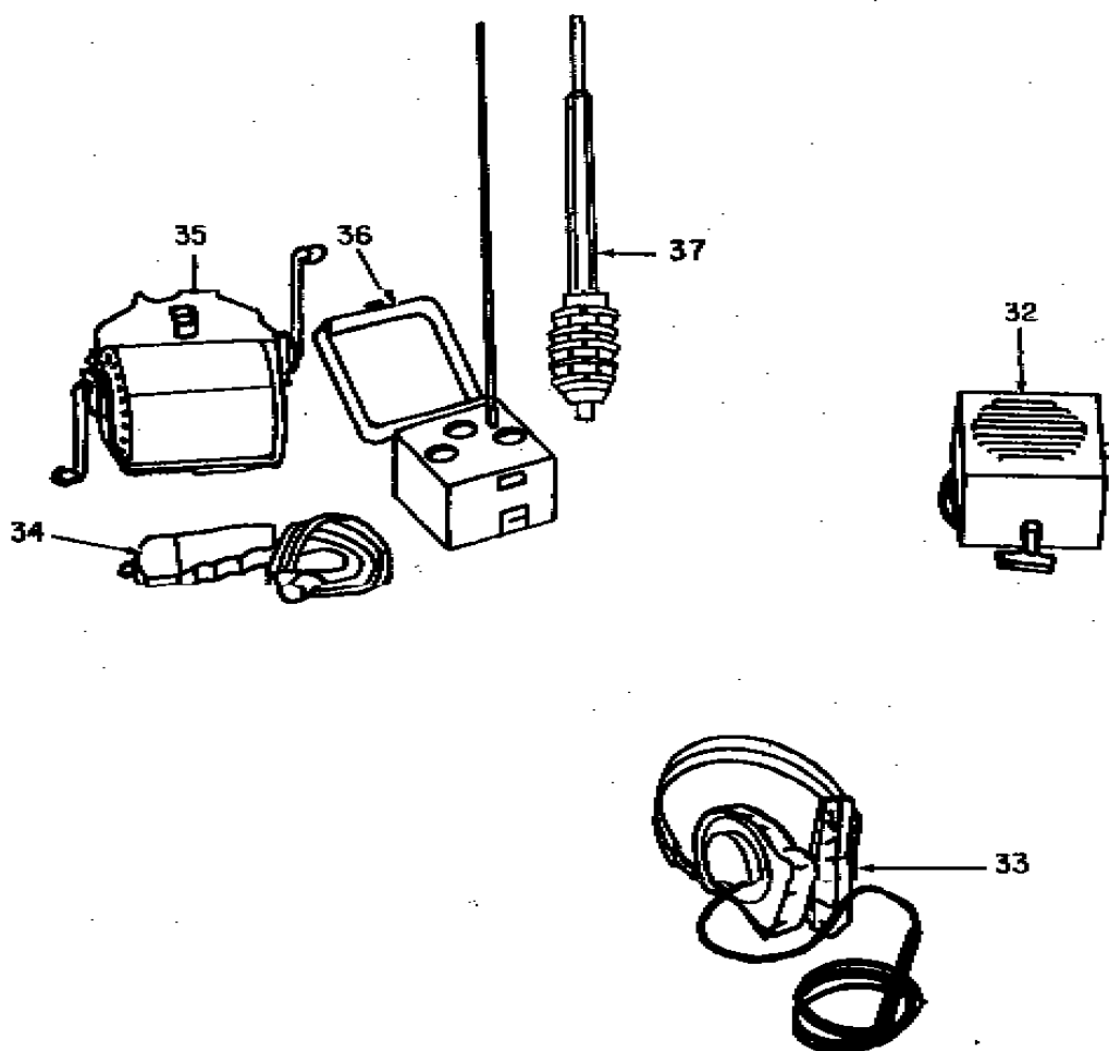
Figure 1. Radio Sets AN/GRC-87, AN/VRC-34(Sheet 2 of 2) .
