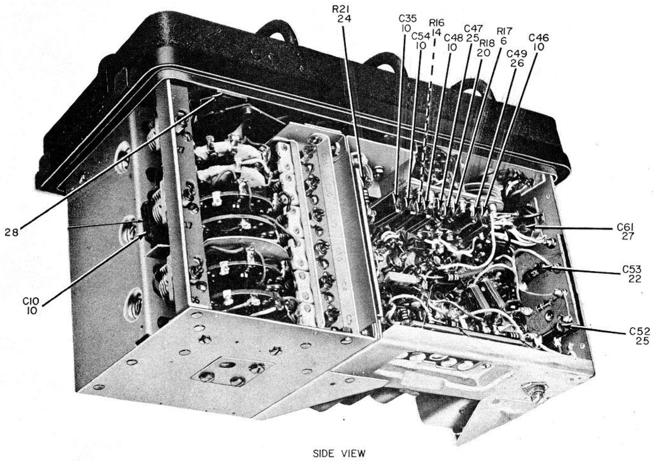
Figure 5 ③ Receiver-Transmitter RT-77/GRC-9, RT-77A/GRC-9 (Sheet 3 of 6).
