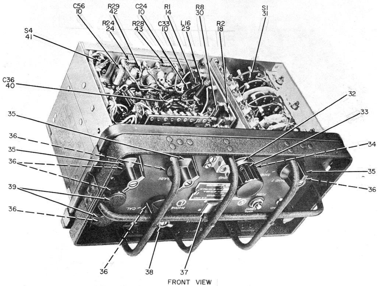
Figure 5.④ Receiver-Transmitter RT-77/GRC-9, RT-77A/GRC-9 (Sheet 4 of 6).
