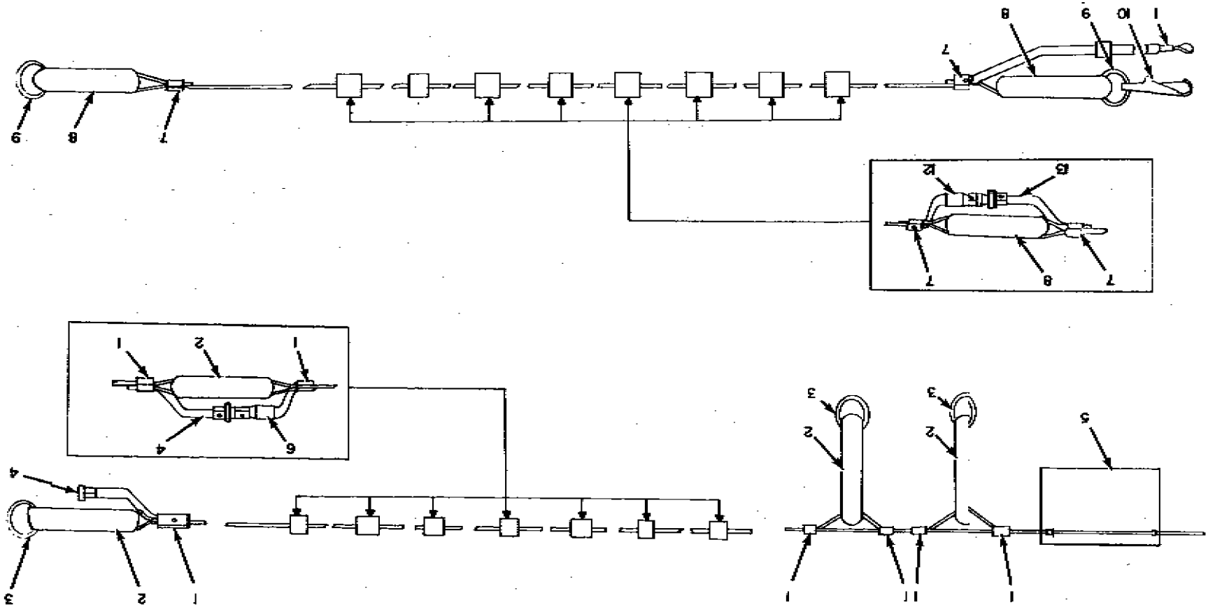
Figure 2. Antenna Assemblies AT-101/GRC-9, AT-102/GRC-9
