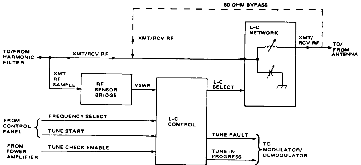
Figure 3-9. Antenna Tuner Block Diagram
