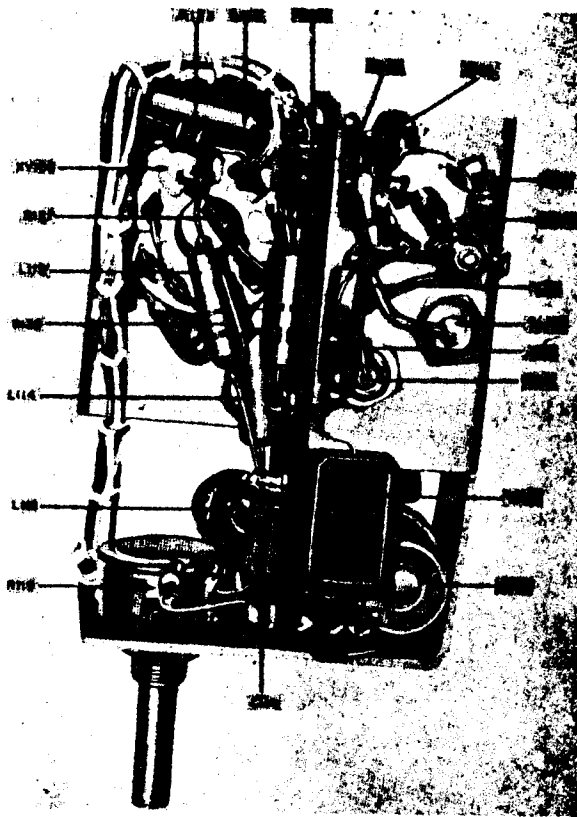
Figure 6-7. Bottom View of Buffer - Amplifier Unit
