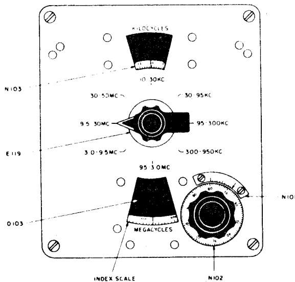
Figure 4-2. Diagram Showing Vernier Reading of Frequency Scale
