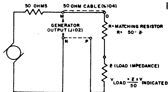
Figure 4-6. Equivalent Circuit of RF OUTPUT X-MULT (J102) with Series Matching Resistor Added
