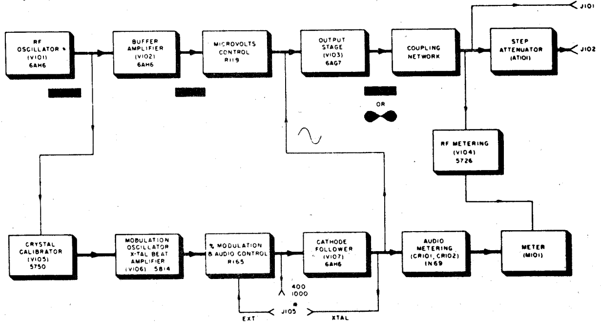
Figure 2-1. RF Signal Generator SG-85/URM-25D, Functional Block Diagram
