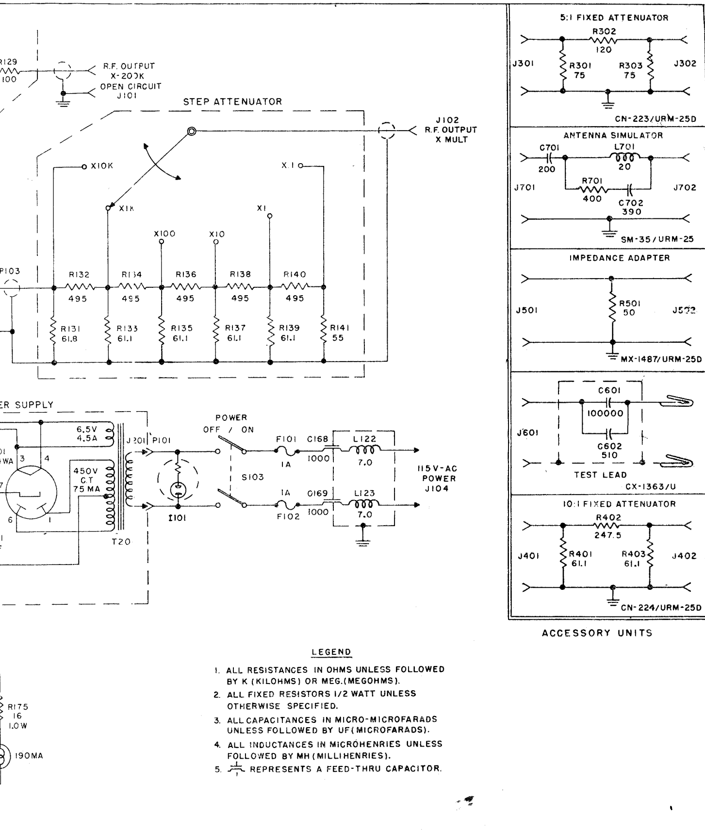
Figure 6-24. RF Signal Generator Set AN/URM-25D, Overall Schematic Diagram
