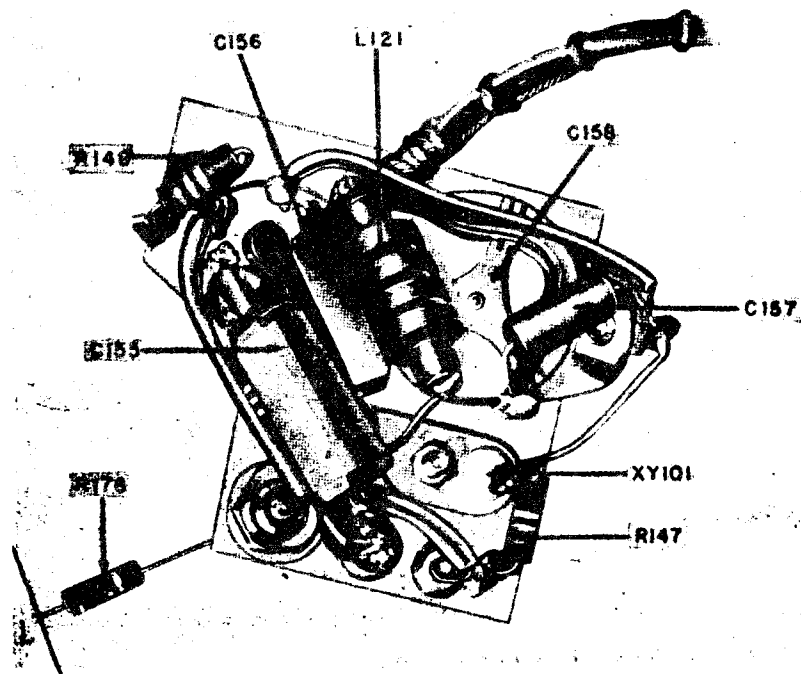
Figure 6-9. Top and Bottom Views of Crystal Calibrator Bracket
