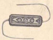
WIRE-WOUND 1W RESISTOR
