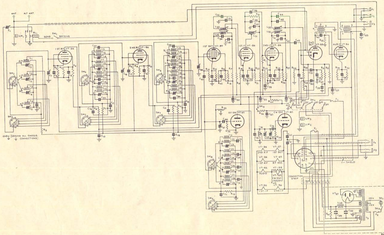
FIGURE 10, RADIO RECEIVER BC-344-D, CIRCUIT DIAGRAM.
