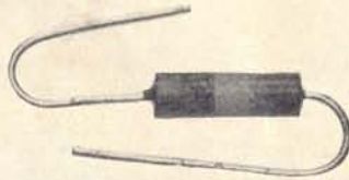
CARBON 1/2 W RESISTOR
