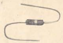
CARBON 1/3W RESISTOR
