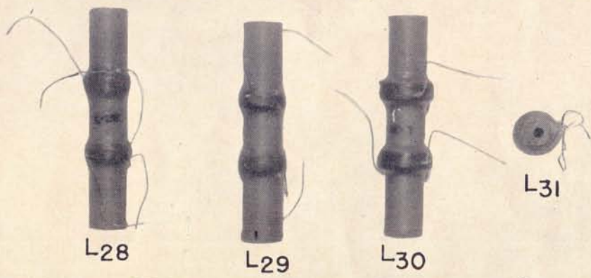
L32 LM1 LM2 WIRE-WOUND 1w RESISTOR CARBON 1/2w RES. CARBON 1/3w RES.
