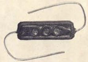
WIRE-WOUND 1W RESISTOR
