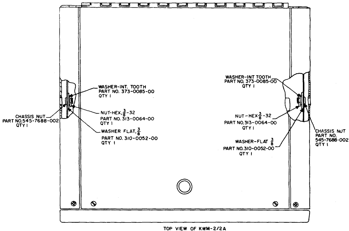
TOP VIEW OF KWM-2/2A
