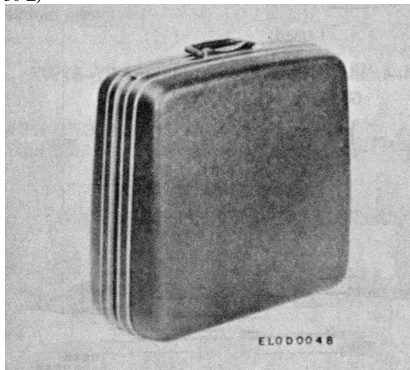
Figure 14-4. Case ,Electrical Equipment CY-6197/GRC-159.
