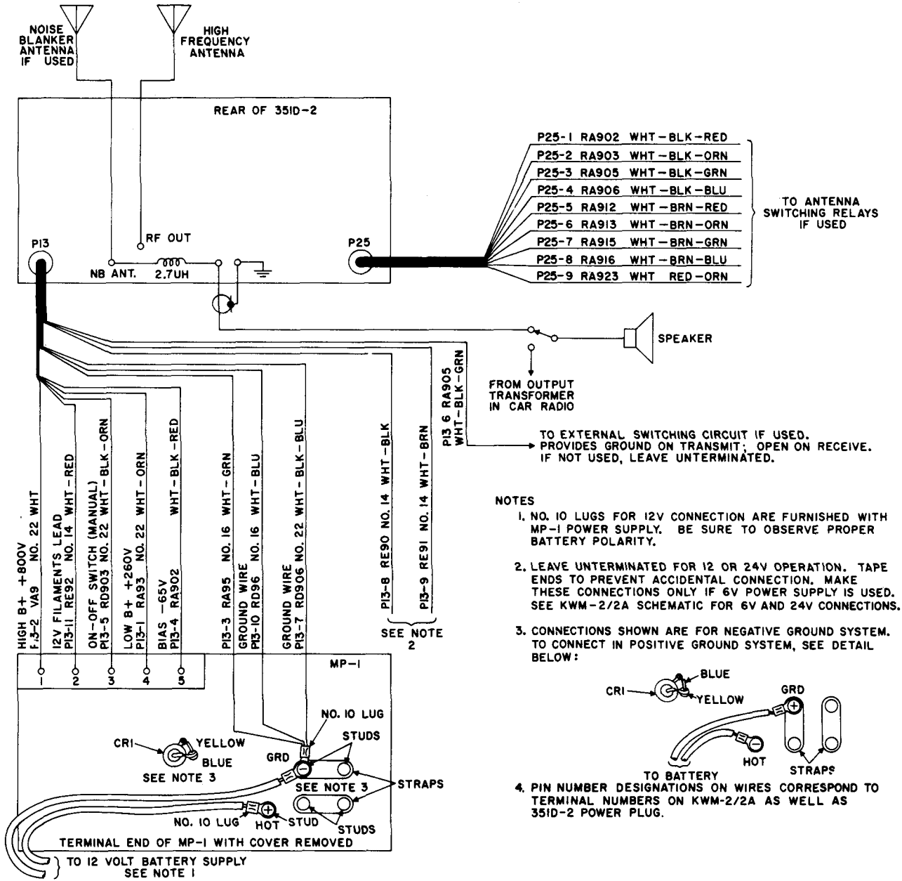
Figure 7-8. Collins MP-1, Collins KWM-2/2A, and Collins 351D-2, mobile interconnection diagram.
