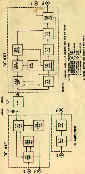
FIG.3 - BLOCK DIAGRAM OF SENDER RECEIVER
