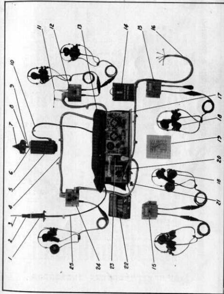
PHOTO 3—INSTALLATION EQUIPMENT FOR RAM II
