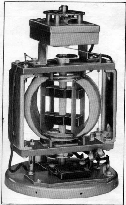
PHOTO 2—INSIDE VIEW OF VARIOMETER
