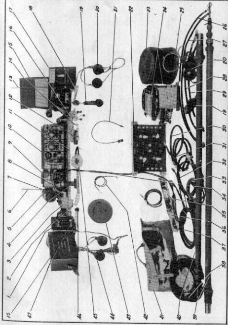
PHOTO 4—INSTALLATION EQUIPMENT FOR GROUND TRUCK STATION
