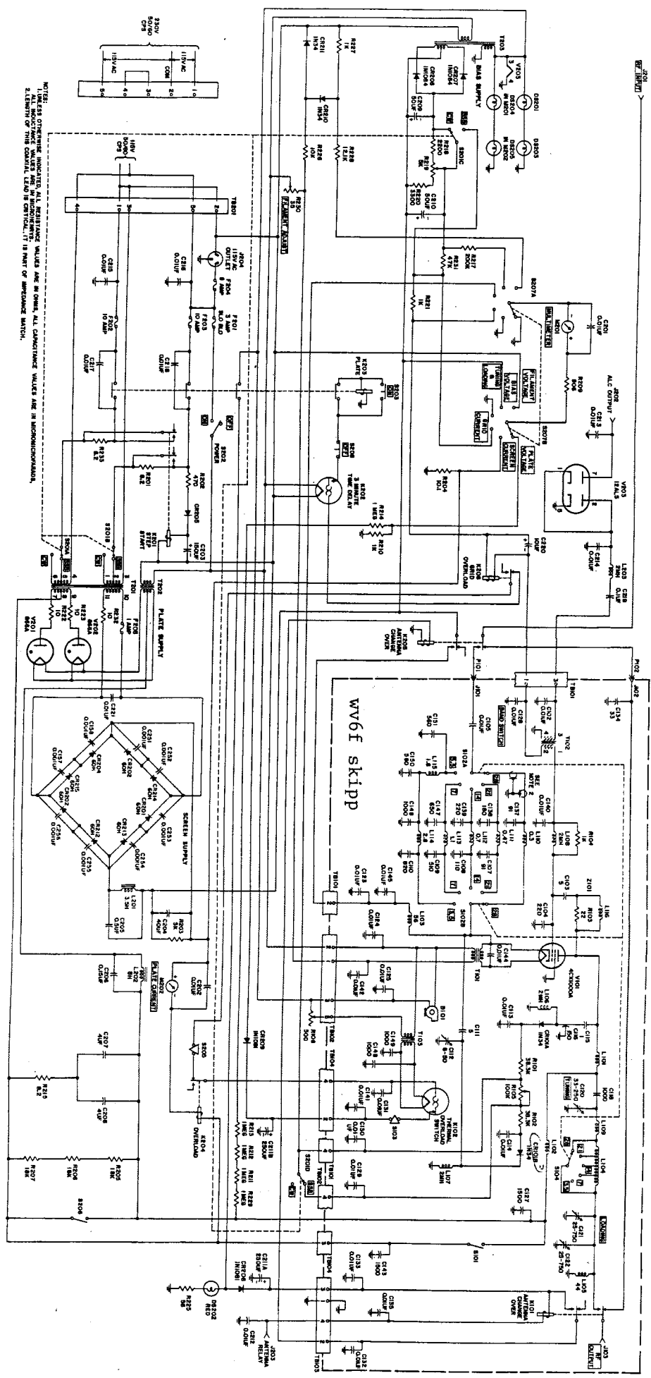
Figure 11. 30S-1 R-F Linear Amplifier, Over-all Schematic Diagram
