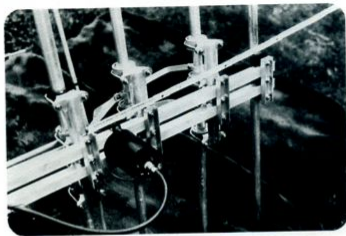
Feed-Point + Balun
