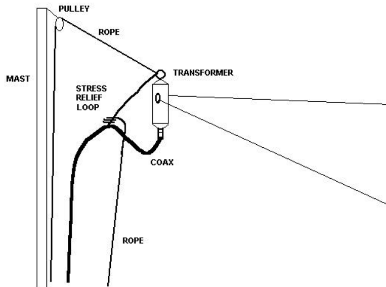
Fig 4-1. Recommended system of halyard and stress relief
