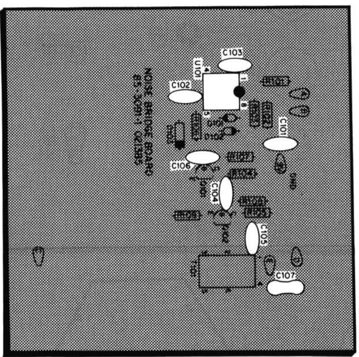
PICTORIAL 1-2
