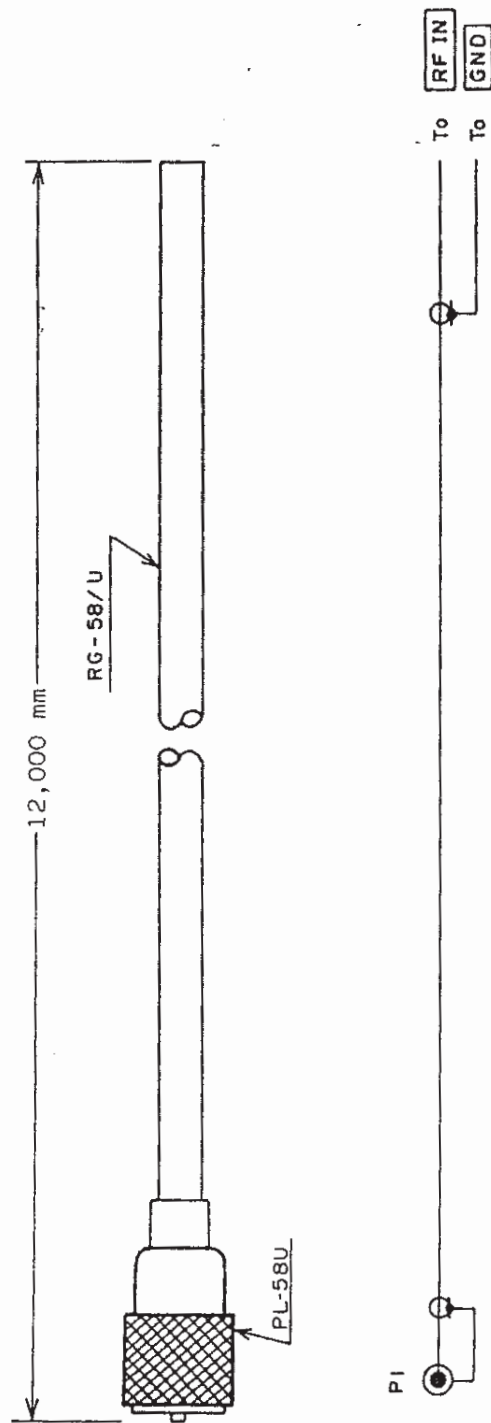
Figure 6-30 RF Cable (CFQ-2859-012) Assembly Drawing
