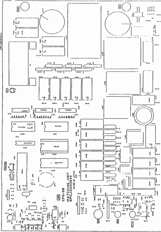
Figure 6-28 Matching Unit (CFG-98) Component Layout
