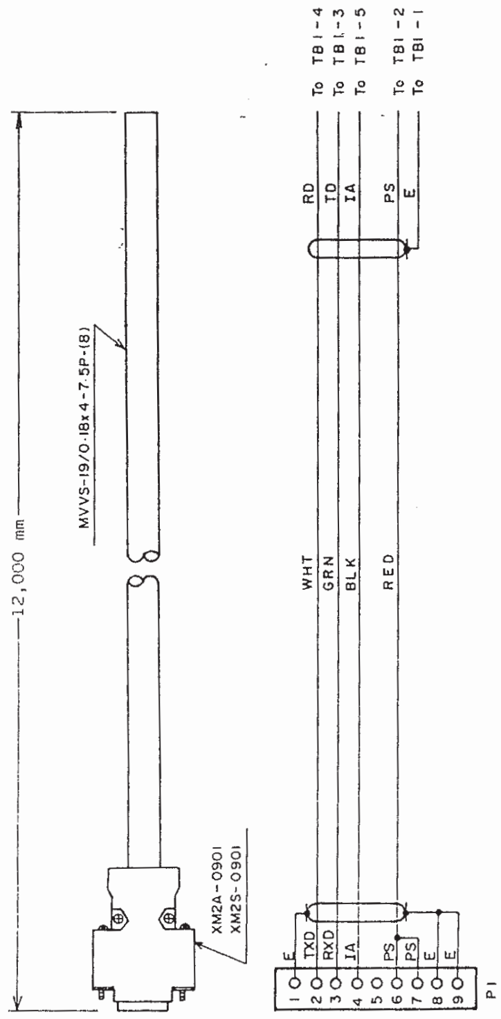
Figure 6-29 Control Cable (CFQ-2858-012) Assembly Drawing
