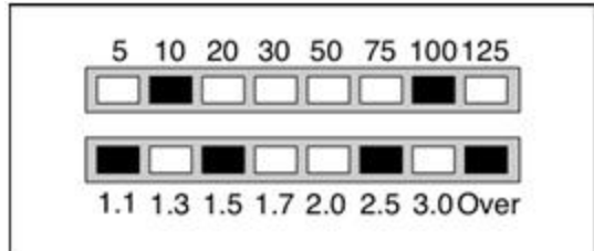
ERR_SWR_PWR: Outer LEDs Toggle
