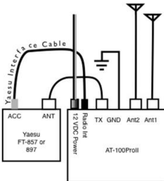
FT-857/897 Installation
