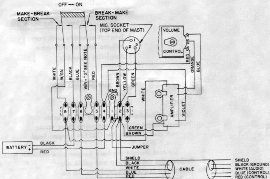
FIG. 2 TU-KIT WIRING DIAGRAM
