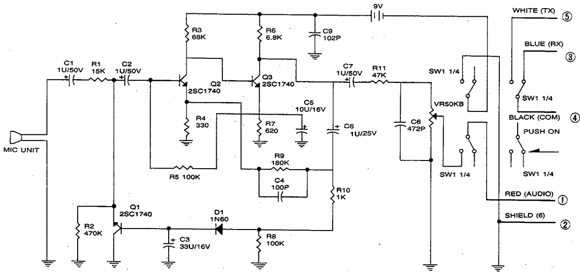
Model CA-72 schematic diagram.
