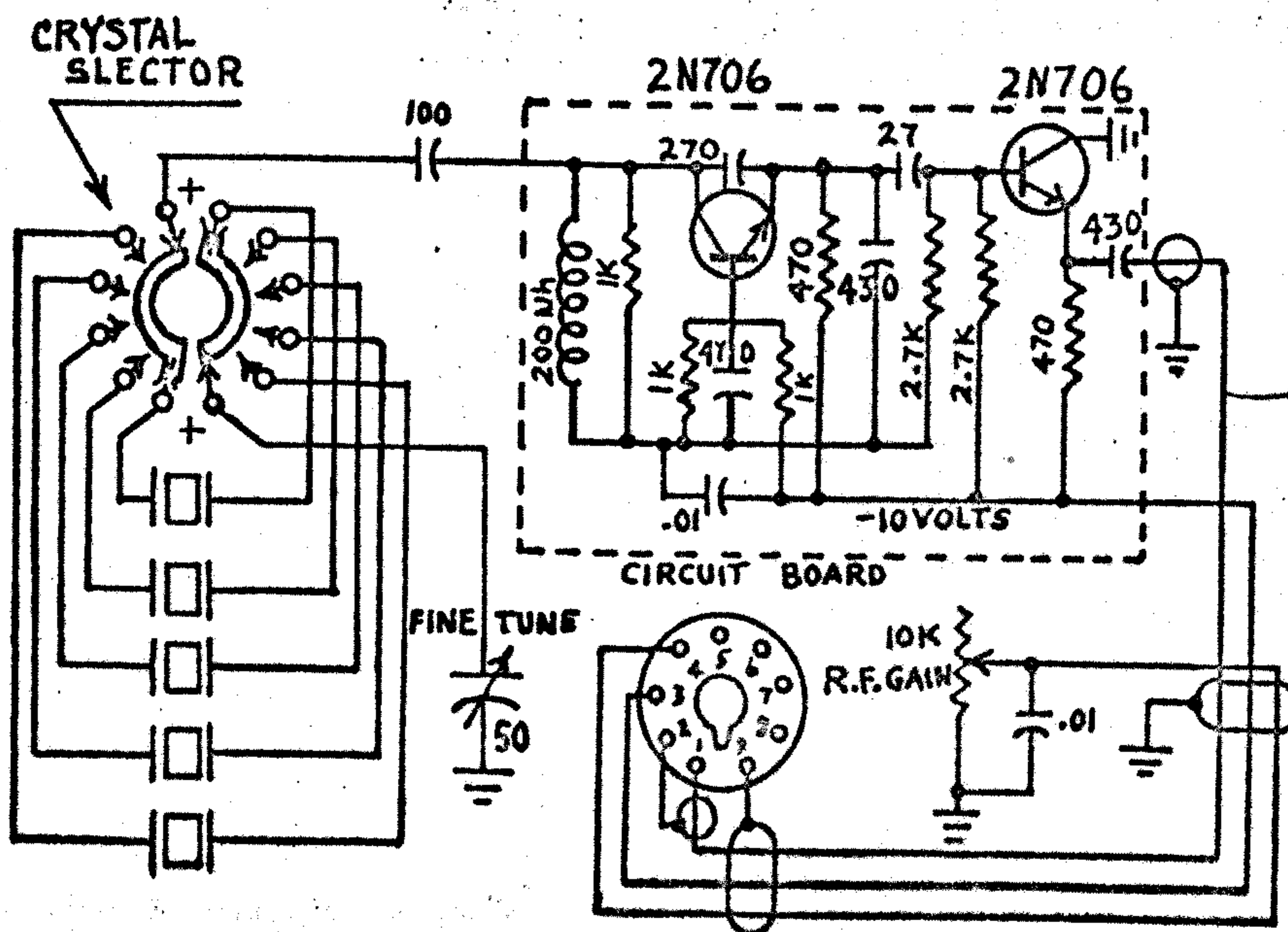
Fig. 7 Schematic Model 405X
