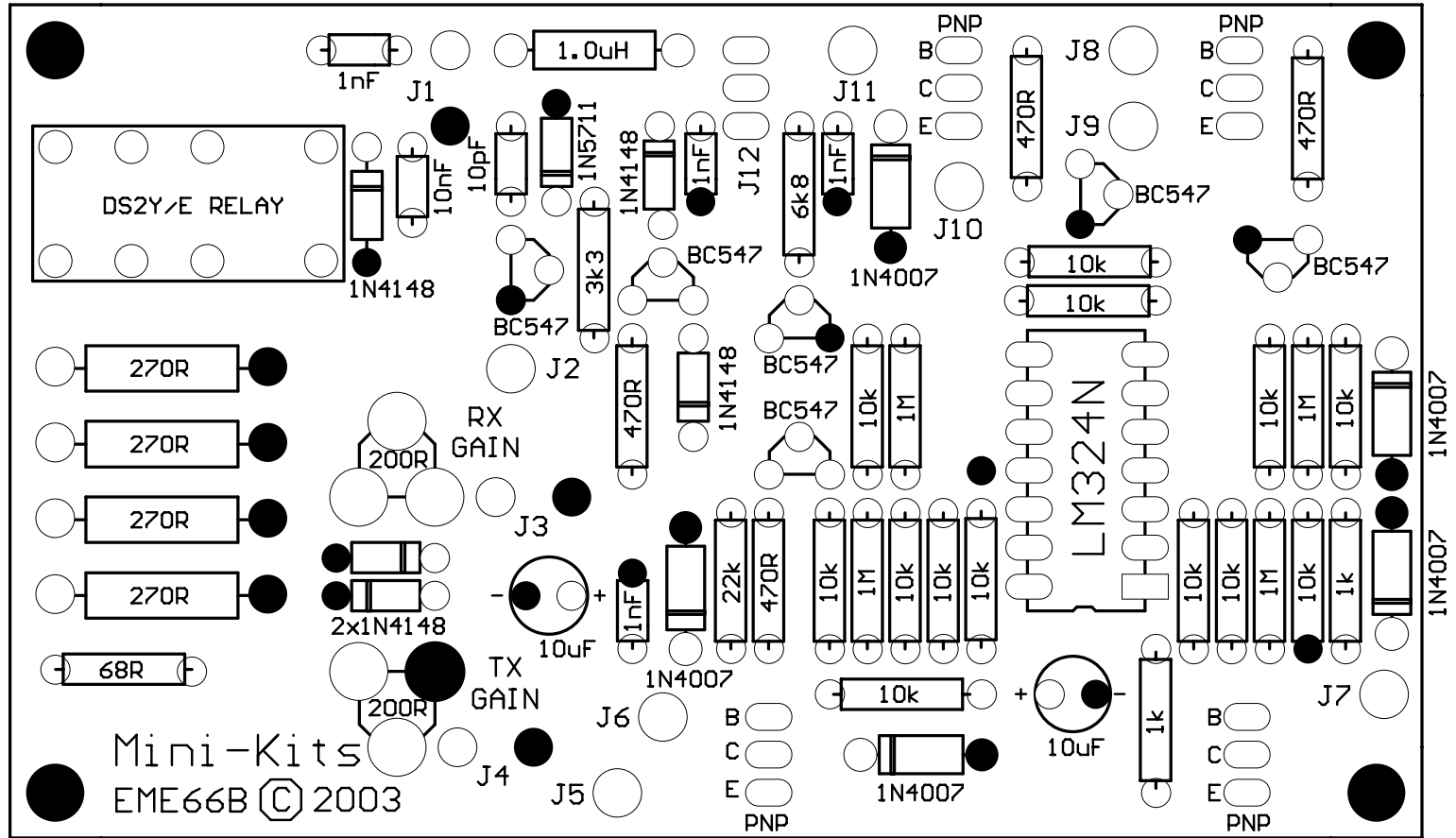
TOP VIEW
