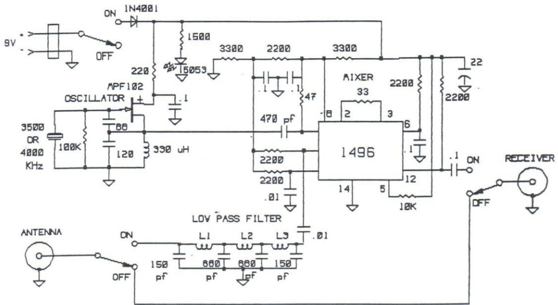
SCHMATIC - VLF CONVERTER
