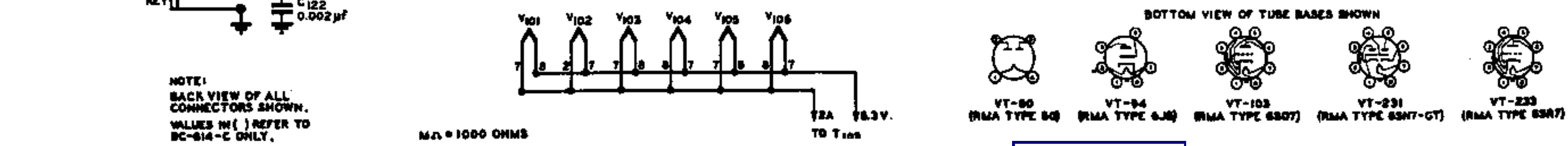
Fig. 4.—Schematic BC-614-A, BC-614-B, BC-614-C.
