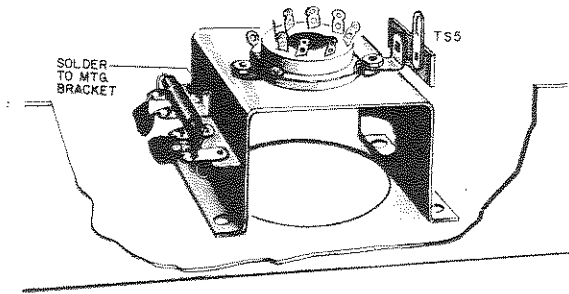
Figure 16. Mounting FR1.
