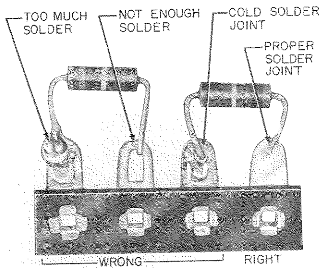
C. SOLDERED CONNECTIONS
