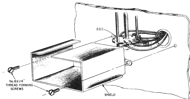
Figure 17. Mounting Shield on S2C.
