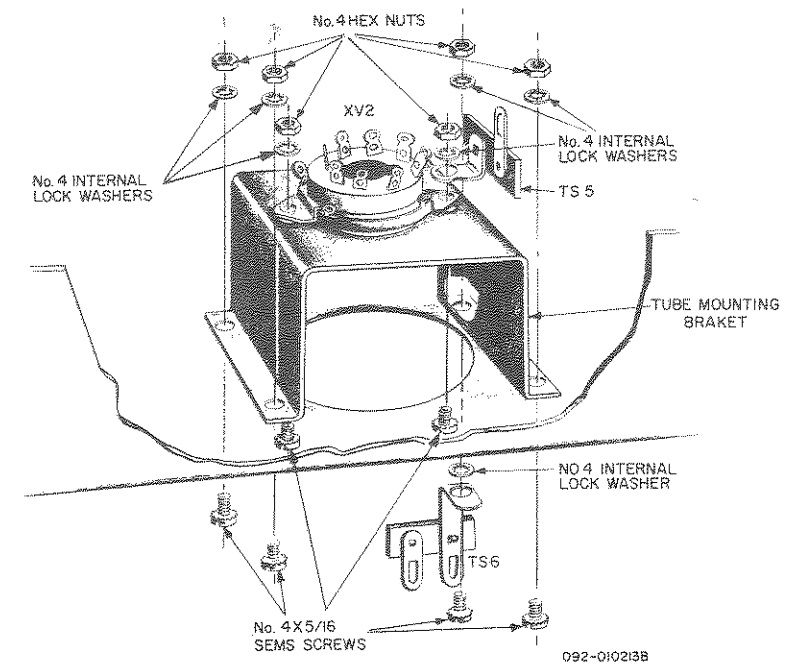
Figure 8. Mounting XV2 and Bracket.
