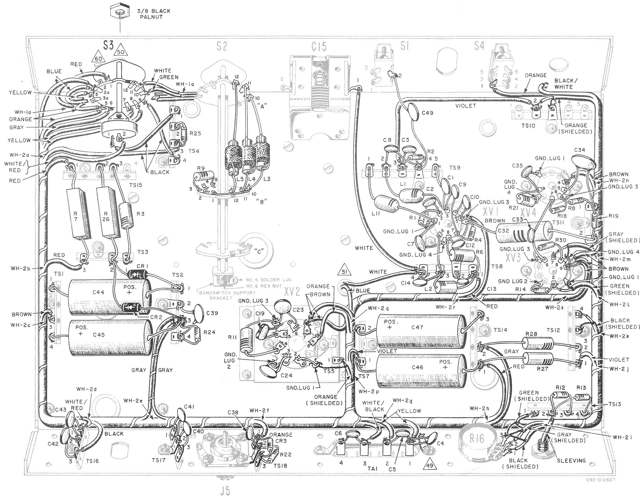
Pictorial 4. Connecting Wiring Harness WH-2 and Components.
