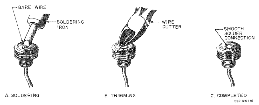
Figure 11. Wiring Microphone Connector.
