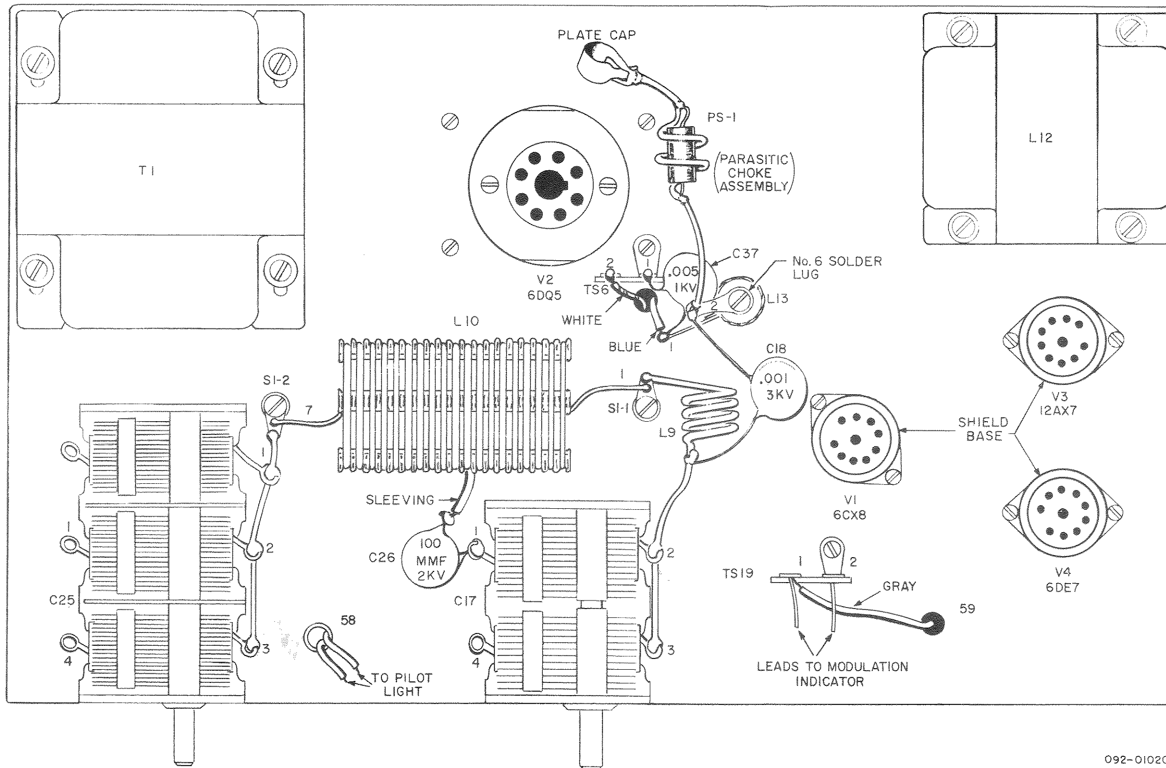
Pictorial 5. Wiring Components on Top of Chassis.
