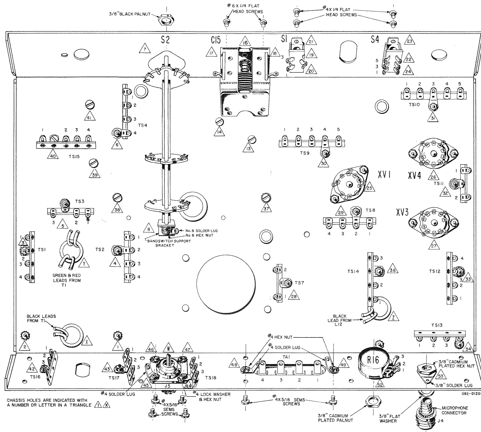
Pictorial 2. Mounting Parts to the Bottom of the Chassis.
