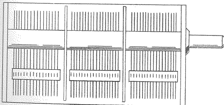
PLATE LOADING CAPACITOR C25
