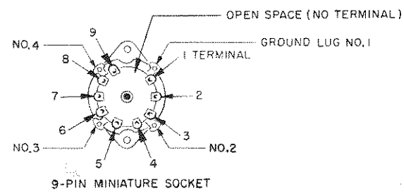
Figure 1. Tube Socket and Shield Base Mounting
