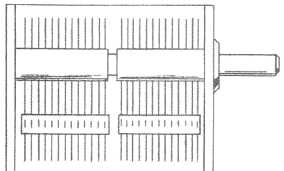
PLATE TUNING CAPACITOR C17
