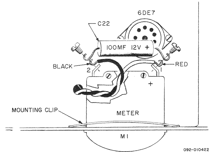
Figure 13. Wiring to Meter M1.
