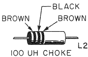
2.5MH PLATE CHOKE
