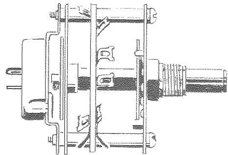
FUNCTION SWITCH S3
