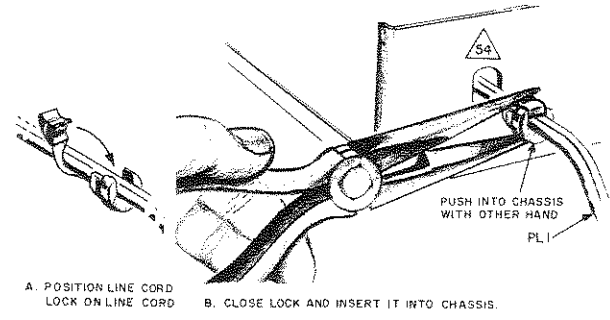
Figure 15. Mounting Line Cord and Lock.
