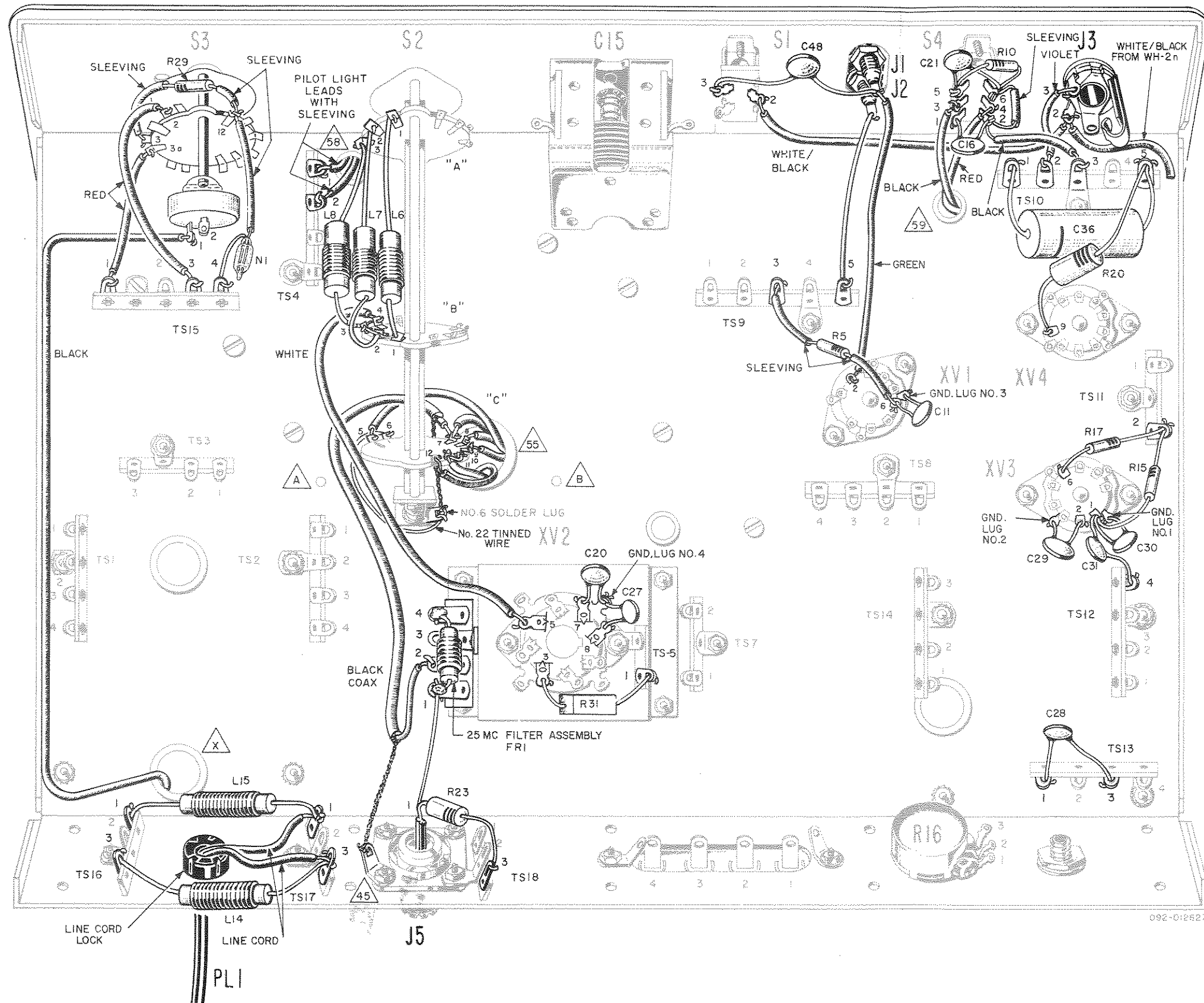
Pictorial 7. Final Component Wiring on Bottom of Chassis.
