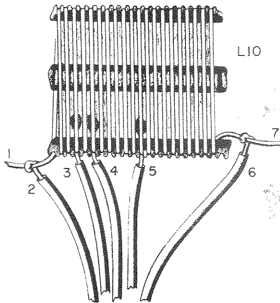
OUTPUT TANK COIL 80 THRU 10 METERS
