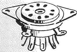
9-PIN MINIATURE SOCKET XV1, XV3, XV4
