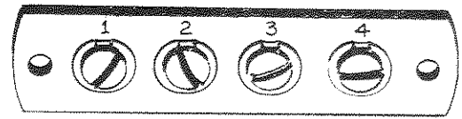
4-CONNECTOR BOARD TA1
