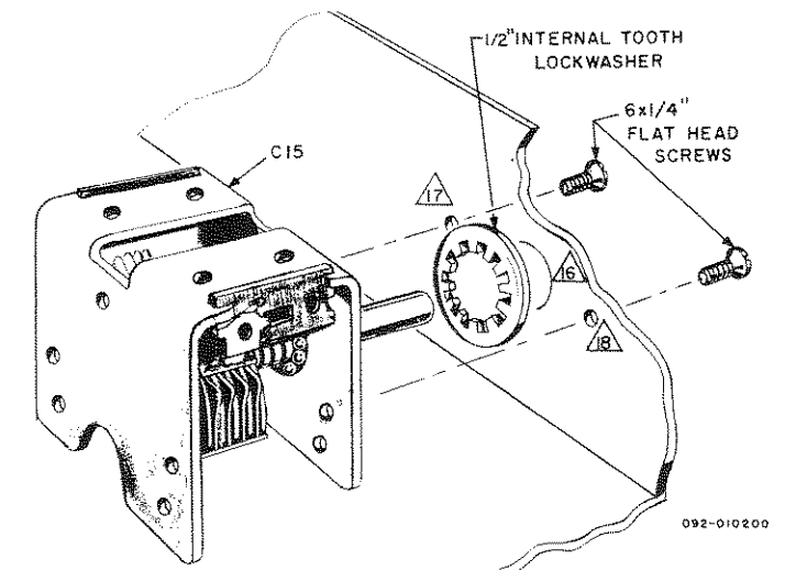
Figure 5. Drive Capacitor Mounting.
