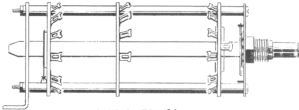
BAND SWITCH S2
