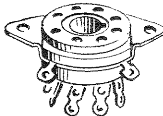
8-PIN OCTAL SOCKET XV2
