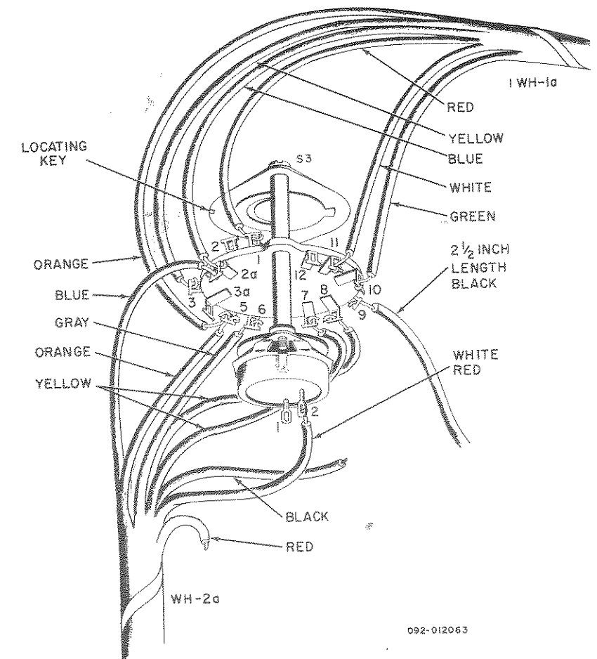
Figure 10. Wiring Switch S3.
