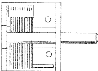
DRIVE CAPACITOR C15
