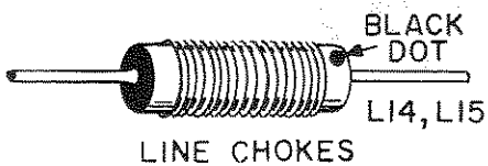
TYPES OF GERMANIUM DIODES (TYPE IN295) DIODES
