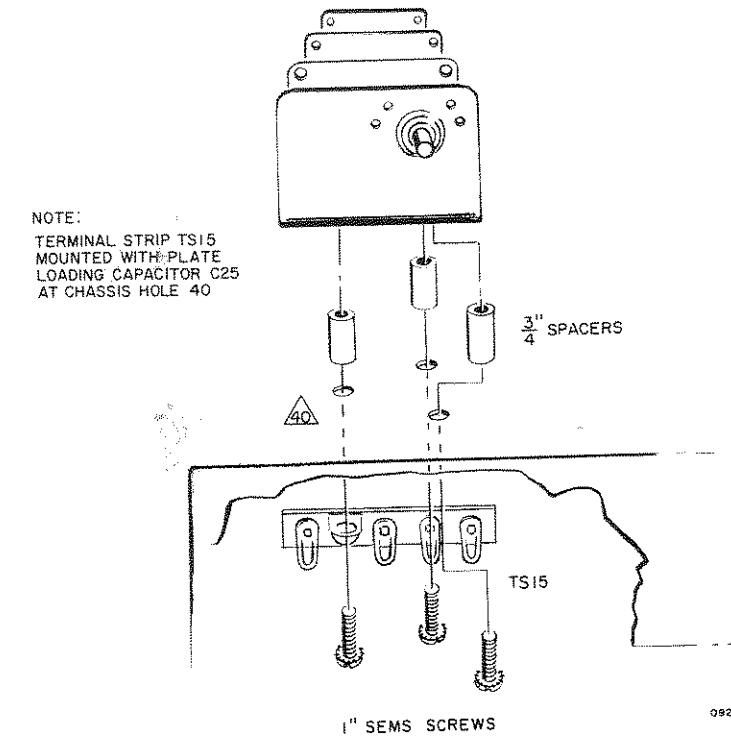
Figure 4. Plate Tuning and Loading Capacitor Mounting.
