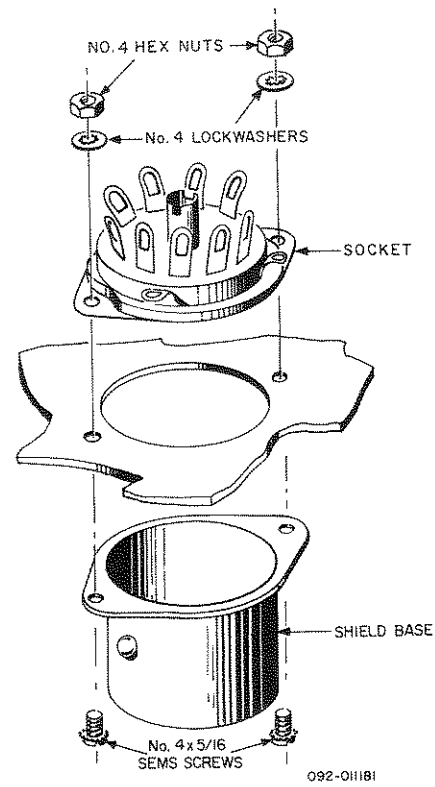
Figure 1. Tube Socket and Shield Base Mounting
