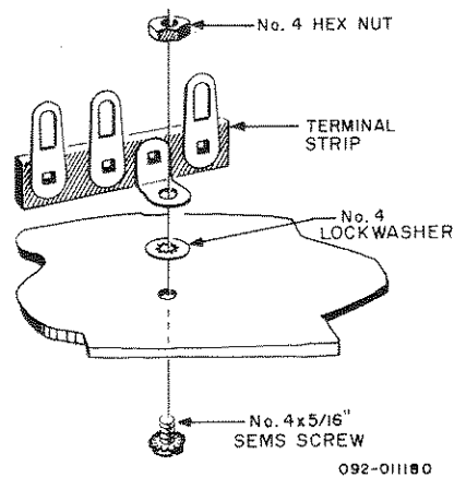
Figure 3. Terminal Strip Mounting.
