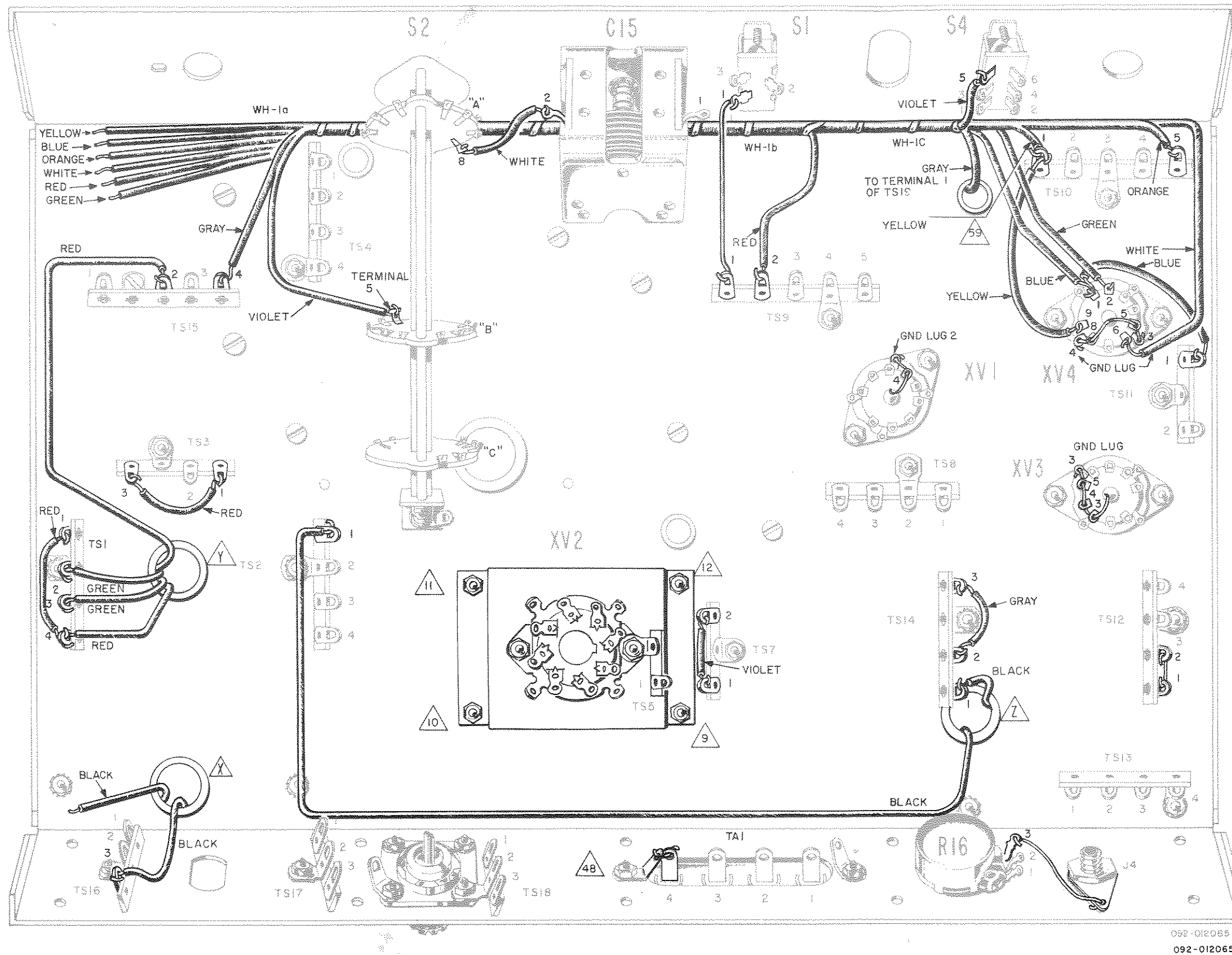
Pictorial 3. Connecting Wiring Harness WH-1.
