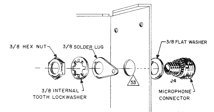
Figure 6. Mounting the Microphone Connector
