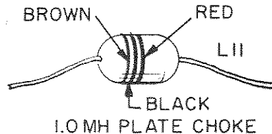
L4 40 METER INTERSTAGE COIL
