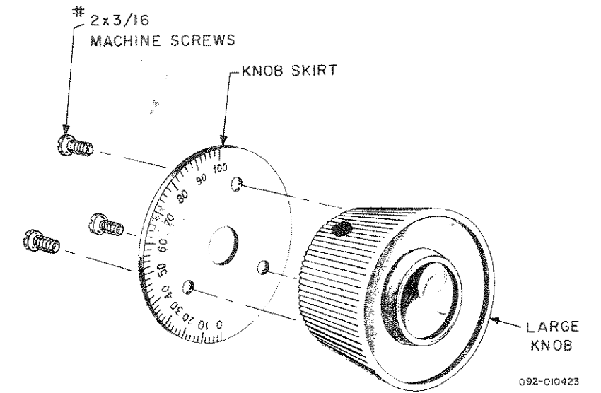
Figure 18. Knob Mounting Detail.
