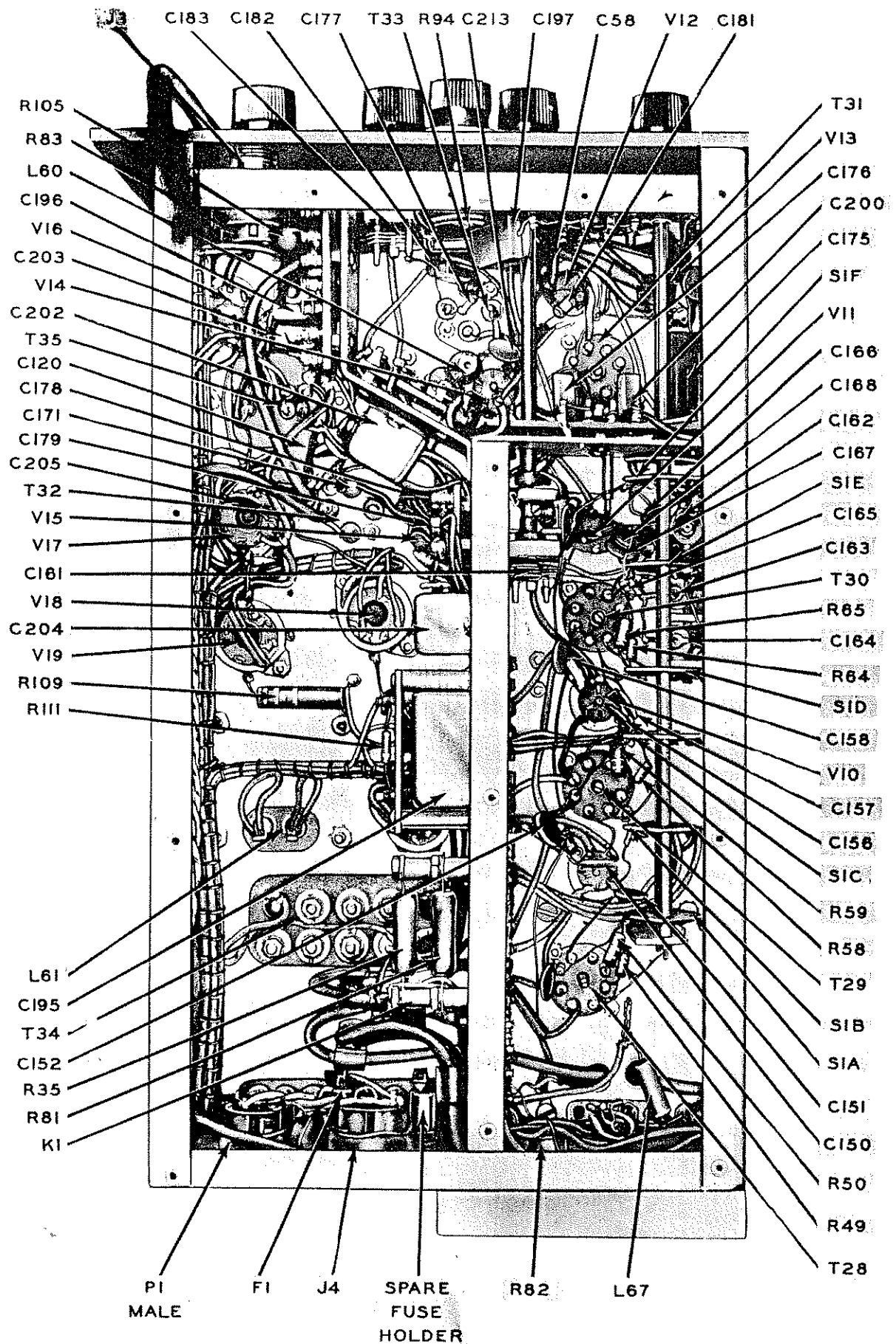
Fig. 14. IF and Audio Chassis, Bottom View
