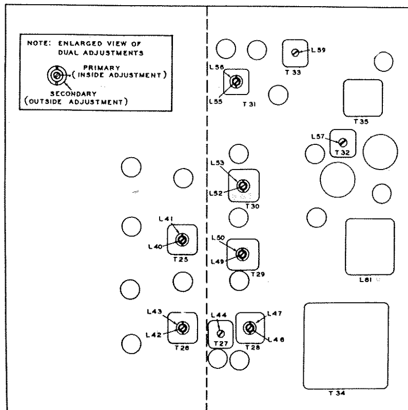
Fig. 8. IF Alignment Diagram
