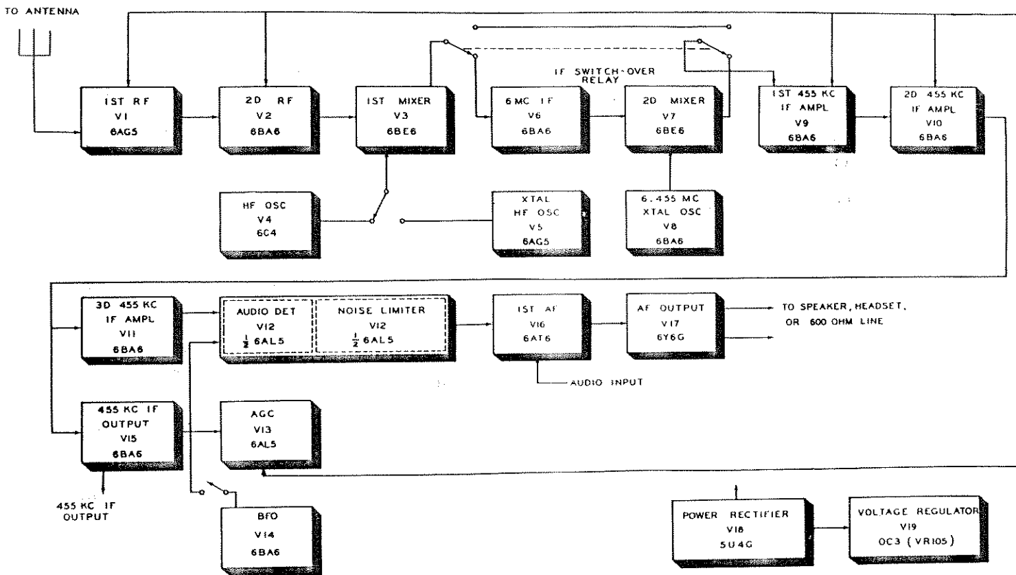
Fig. 4. Block Diagram
