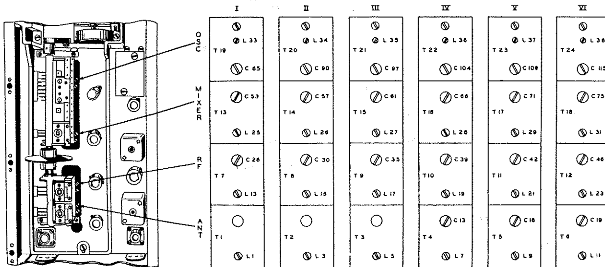
Fig. 9. RF Alignment Diagram
