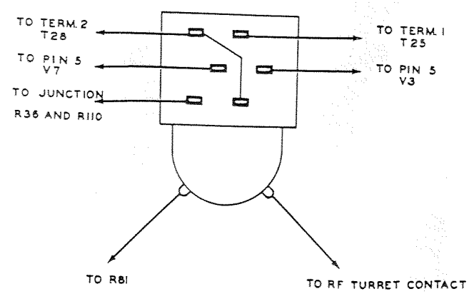
1-f switch-over relay connections.
