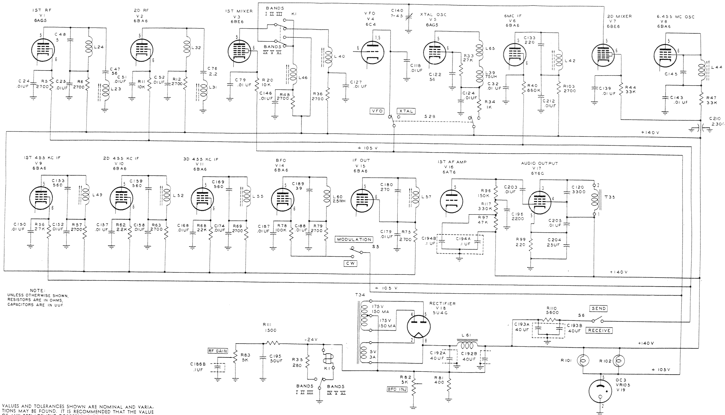
Fig. 18. +B Voltage Distributions
