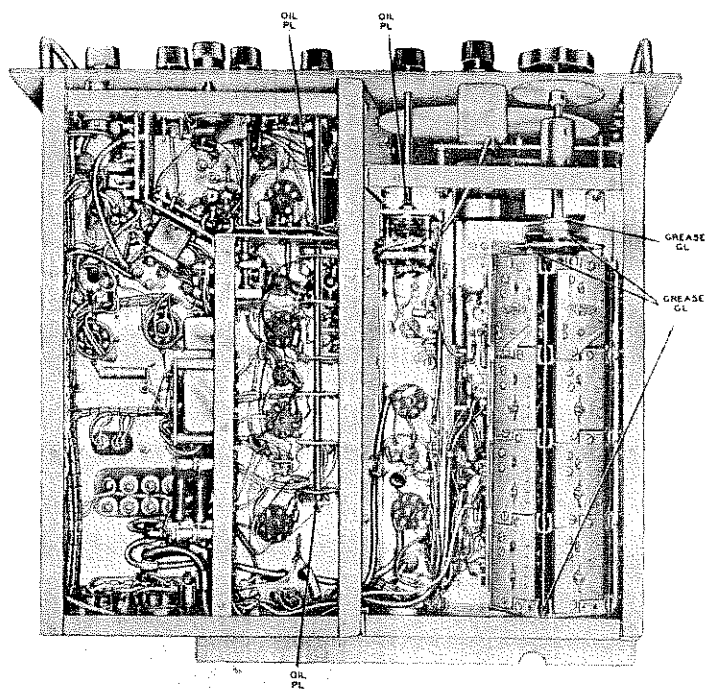
Fig. 6. Lubrication Points, Bottom
