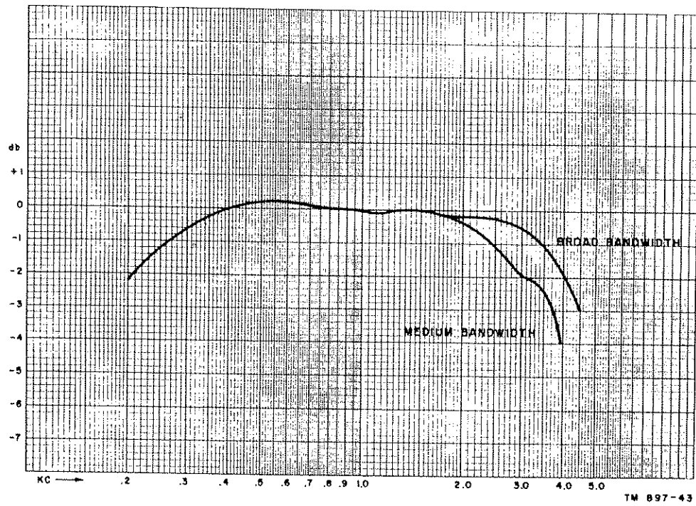
Fig. 11. Typical AF Response Curve
