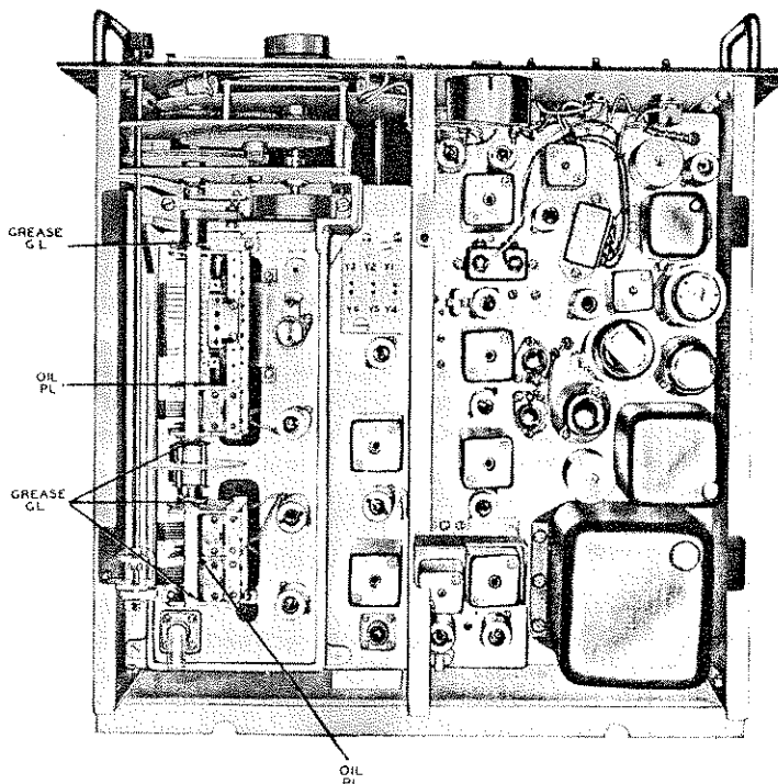
Fig. 7. Lubrication Points, Top
