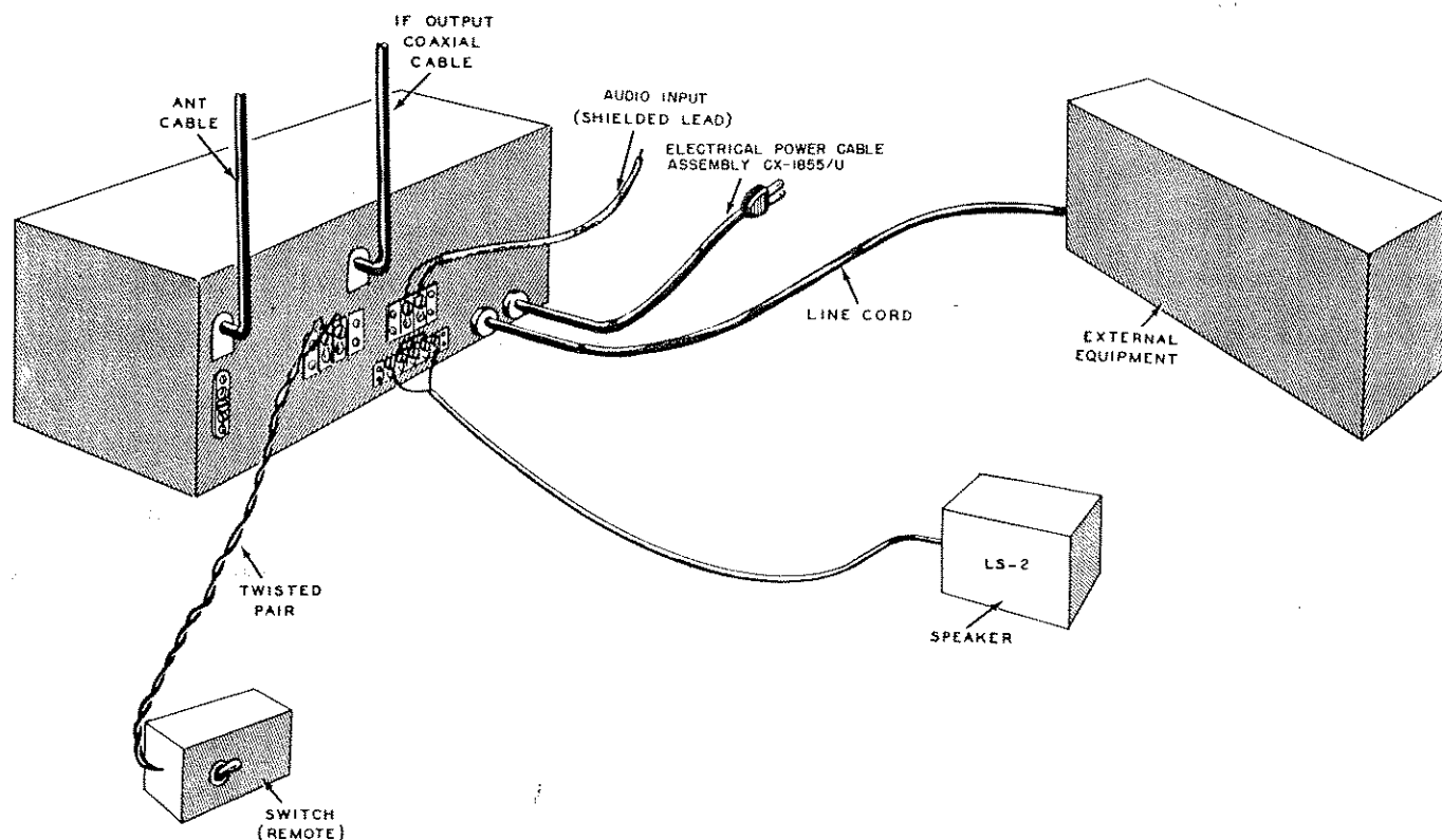
Fig. 2. Connections for Operating
