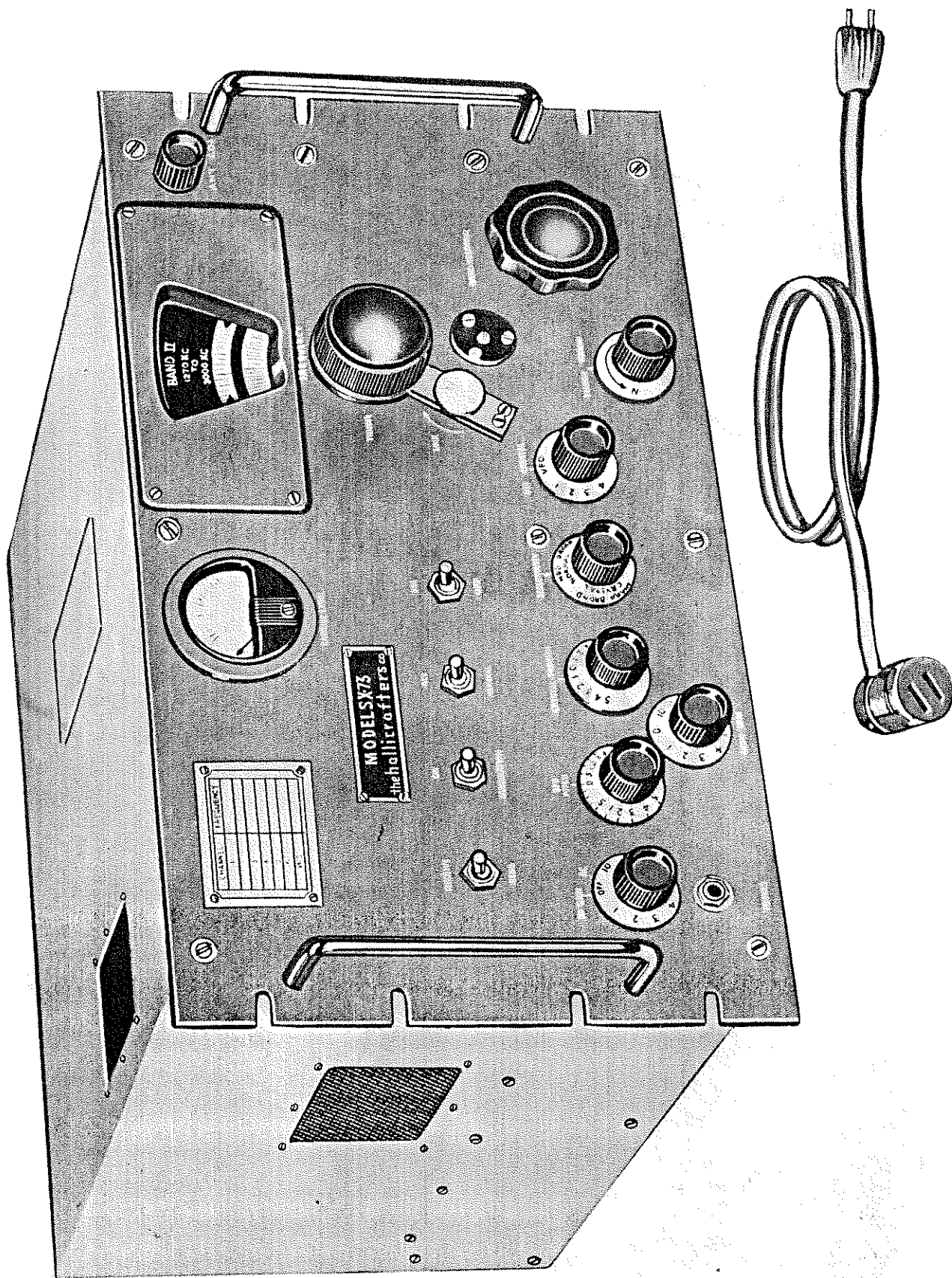
Fig. 1. Hallicrafters Communication Receiver Model SX-73
