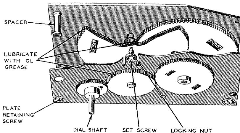
Fig. 5. Lubrication of Dial Drive Mechanism
