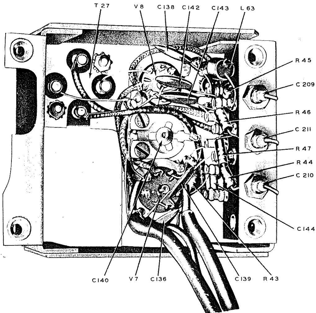
Fig. 12. Second Mixer and 6.455 mc Oscillator Chassis, Bottom View
