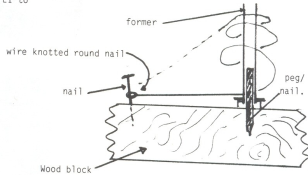
Winding Jig
