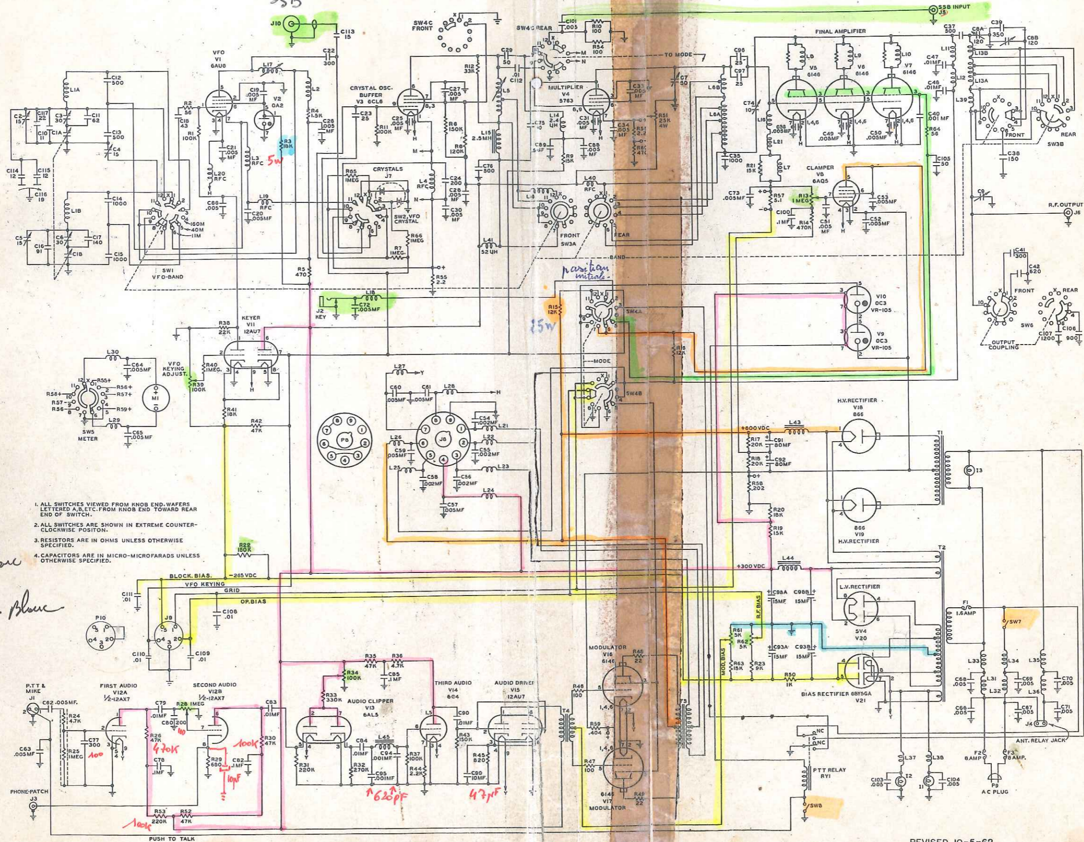
Figure 9, Valiant II Schematic Diagram
