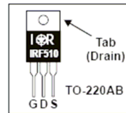
IRF510 FET terminal identification.
