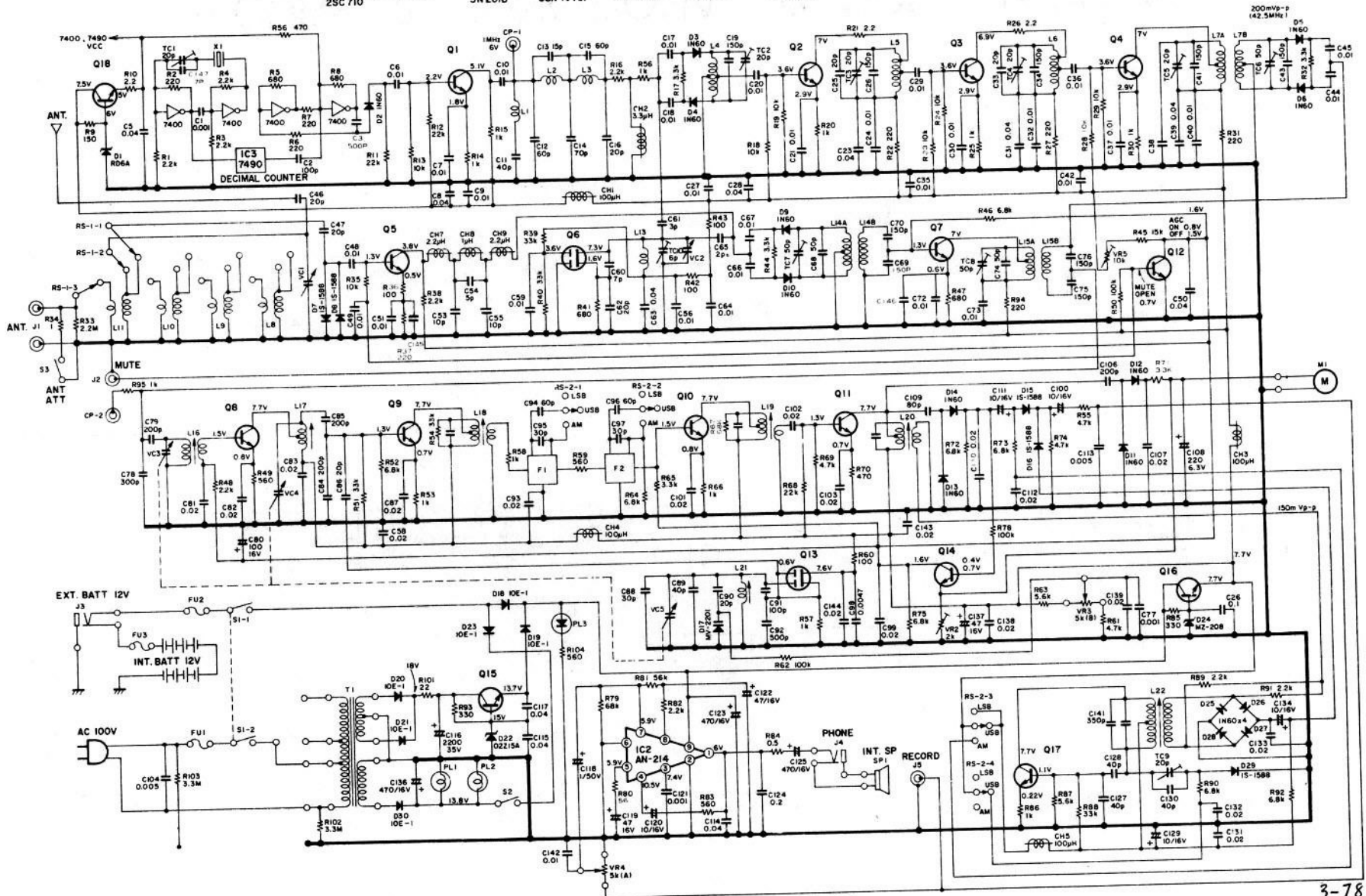
FIGURE 3: SCHEMATIC DIAGRAM
