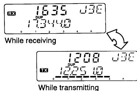
Cross channel operation example
