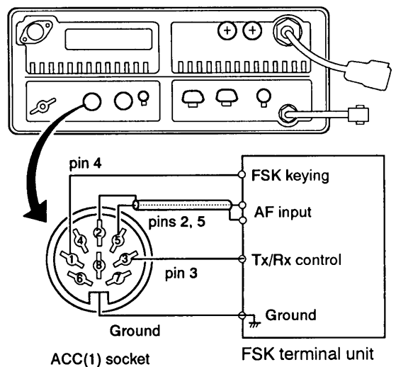
FSK terminal unit connection
