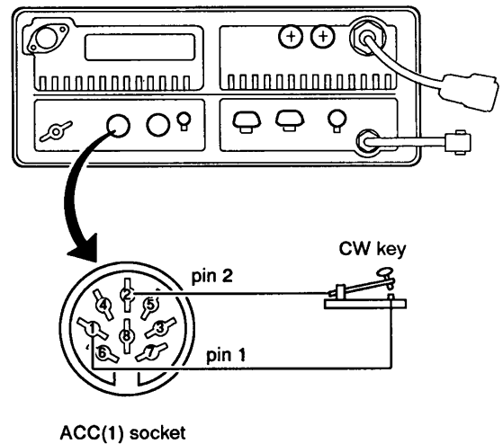
CW key connection
