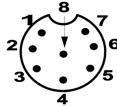
The illustration above shows the pin numbers on the front panel microphone connector.
