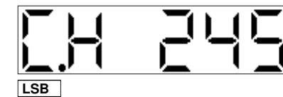
This display shows that the channel in use (Channel 245) is set to LSB mode. Note the LSB label below the display window.
