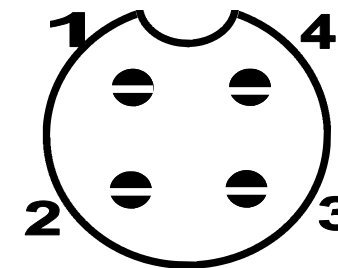
The illustration above shows the pin numbers on the rear panel power connector.
