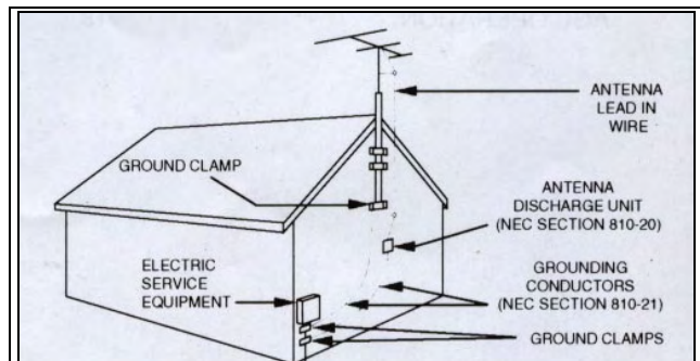
EXAMPLE OF ANTENNA GROUNDING
