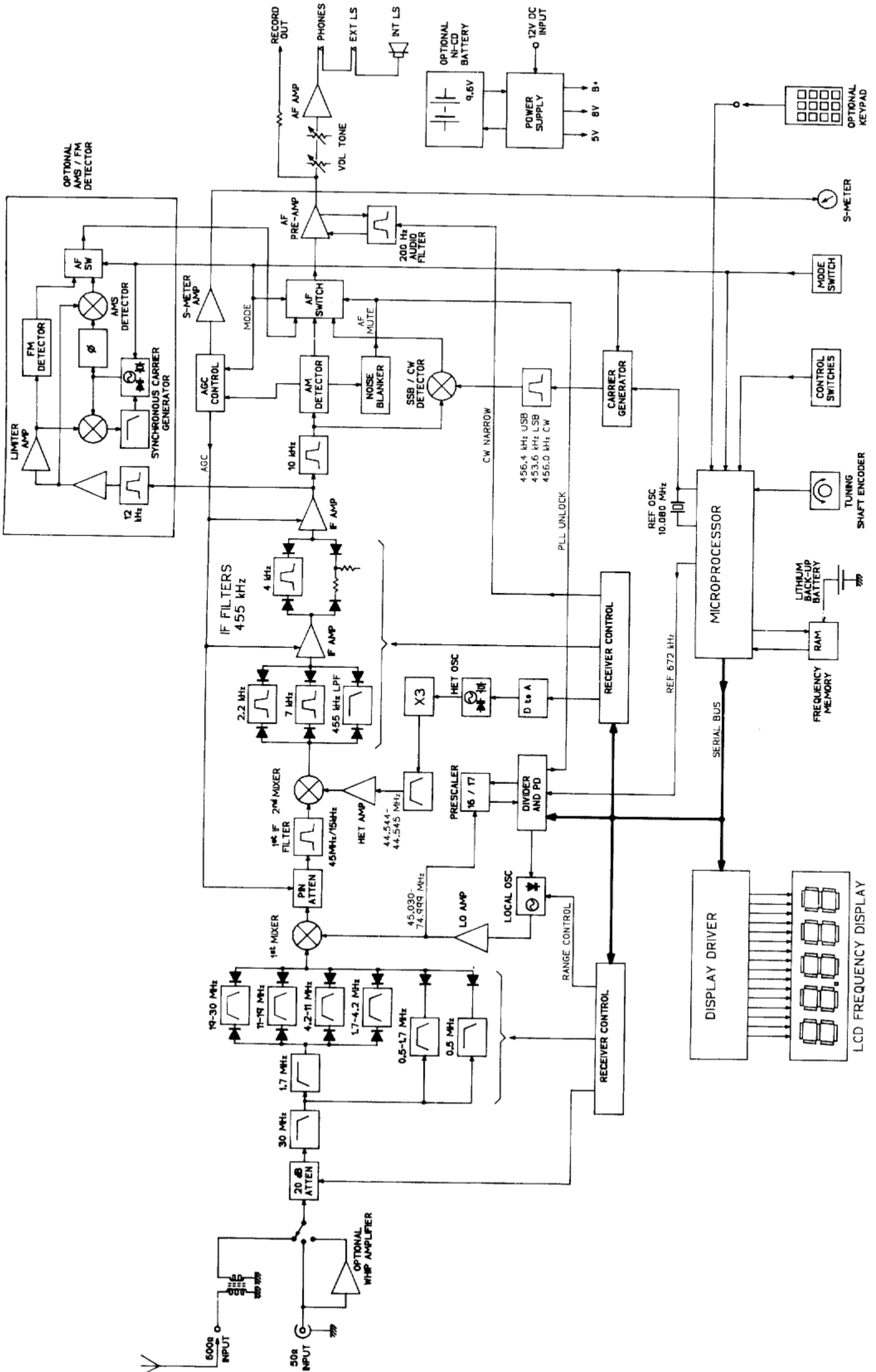
HF-225 BLOCK DIAGRAM
