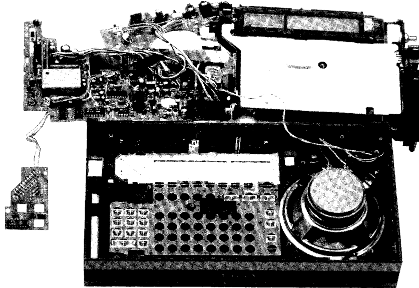
External 4.5V power-supply connection.
