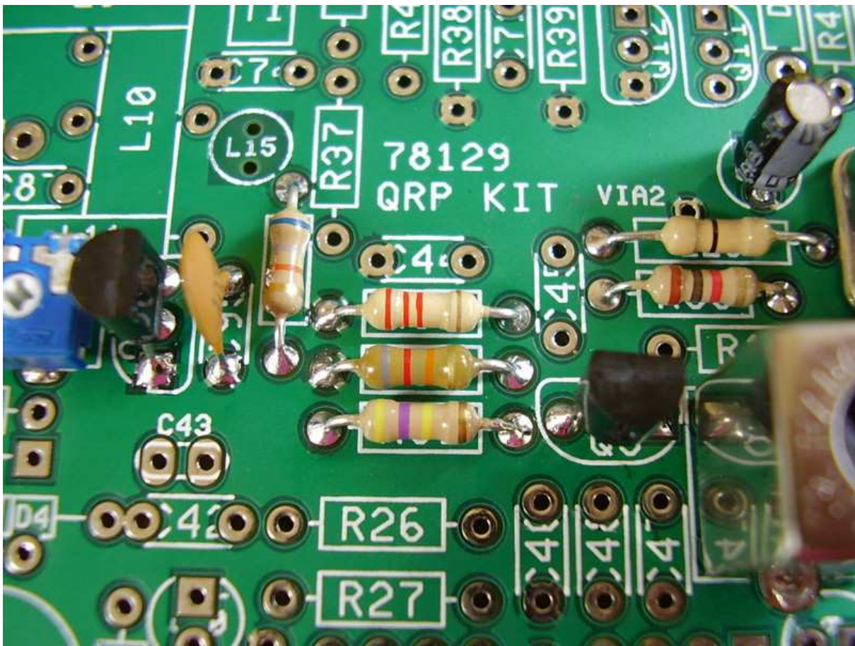
Figure 6.41: [4-40] R31 470K.
