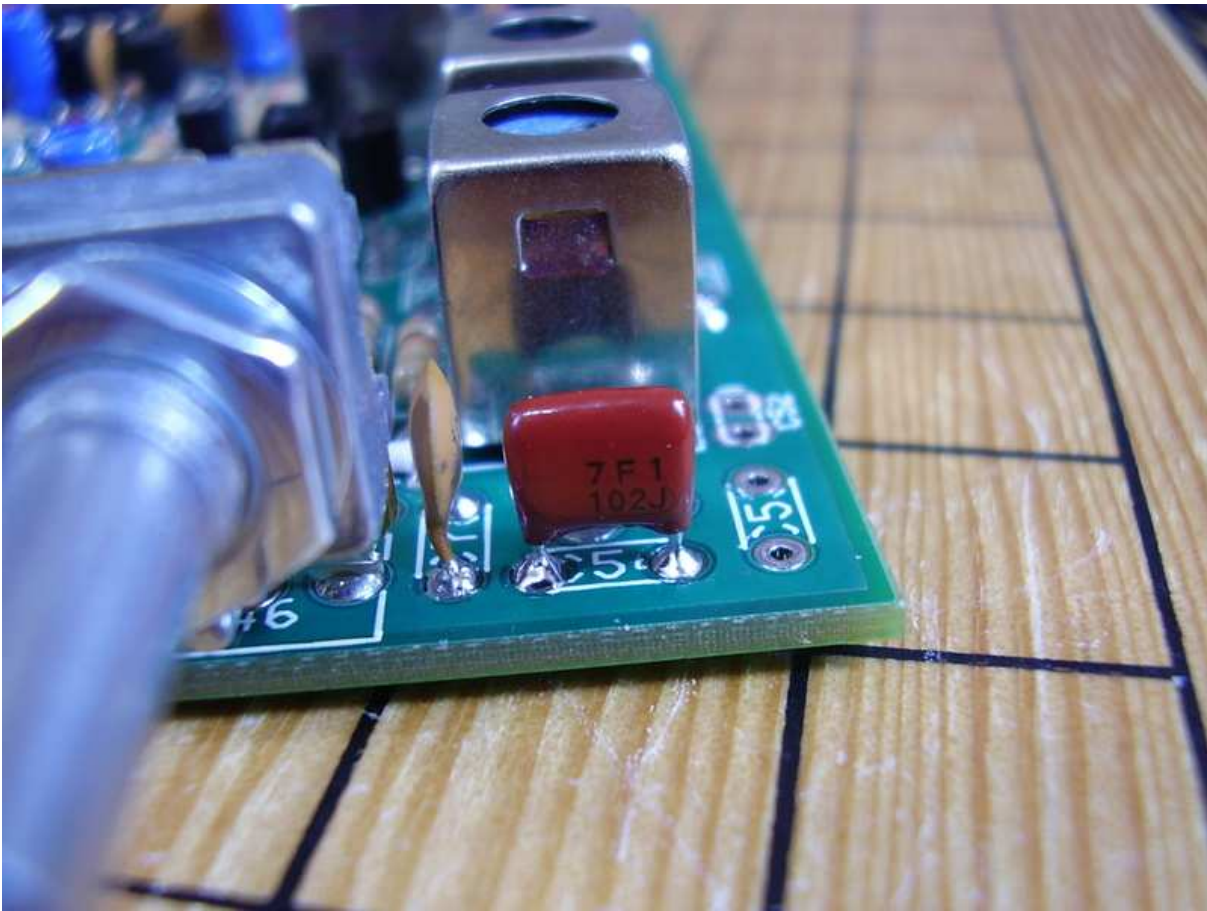
Figure 6.17: [4-14] C54 .001\mu\text{F} .
