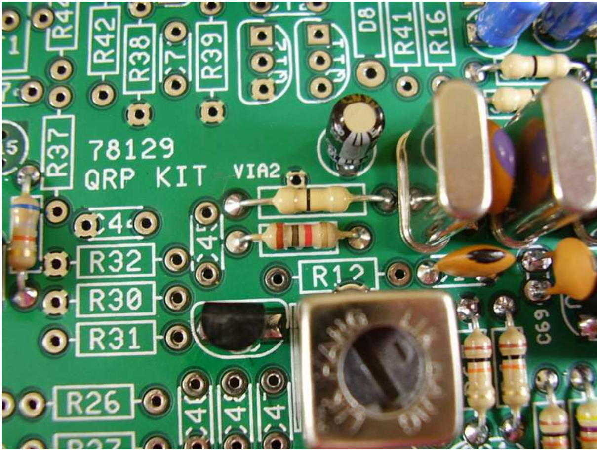
Figure 6.38: [4-37] R33 1K.
