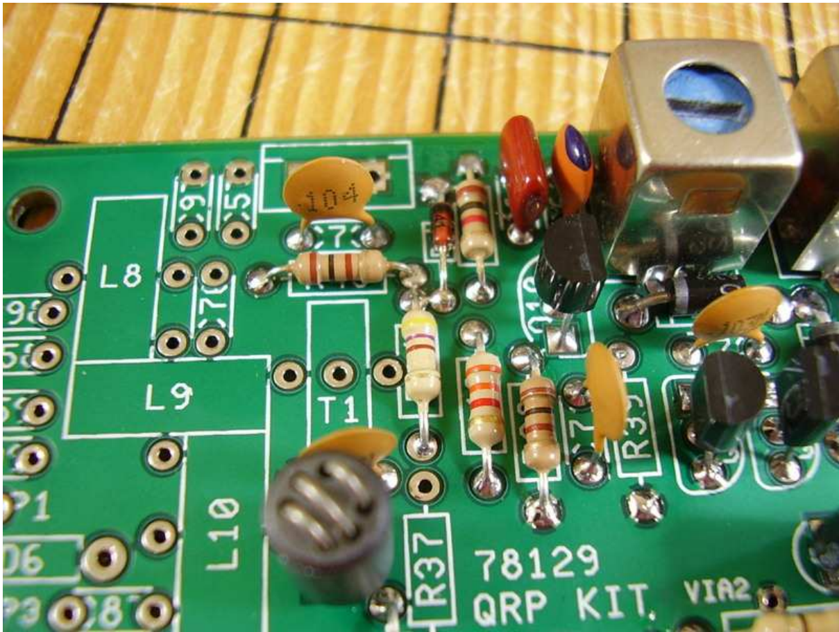
Figure 9.18: [7-19] R44 470 ohms.
