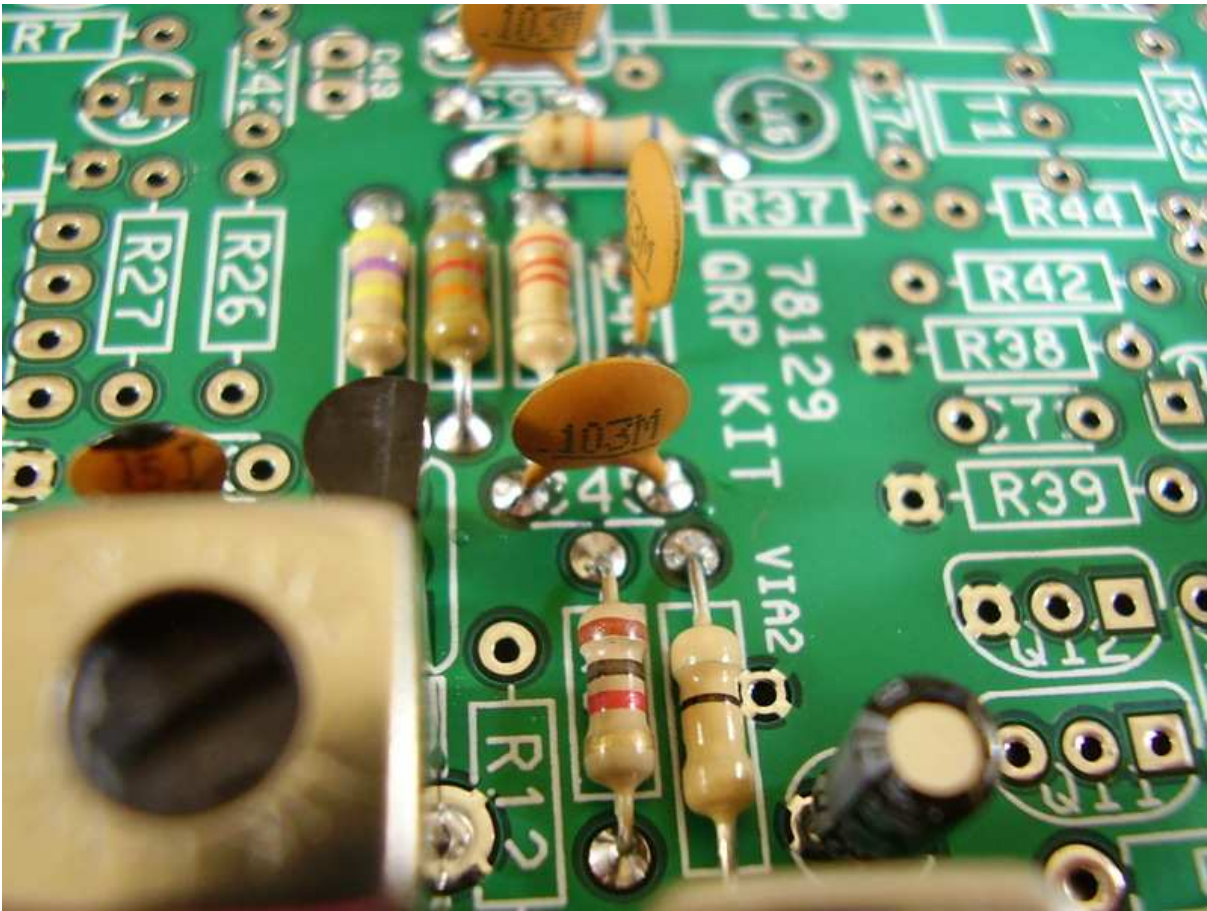
Figure 6.45: [4-44] C45 .01 \mu F.
