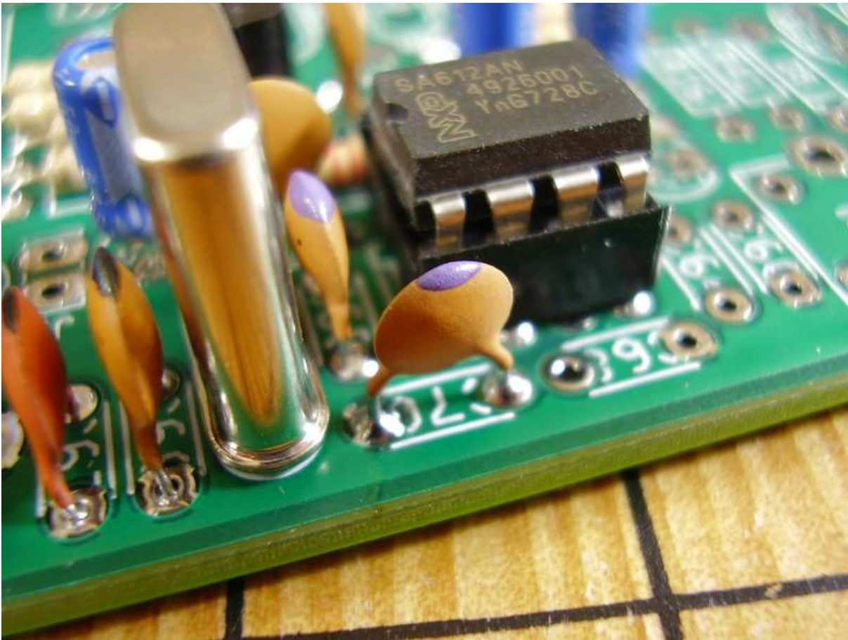
Figure 5.12: [3-9] C70 47pF.
