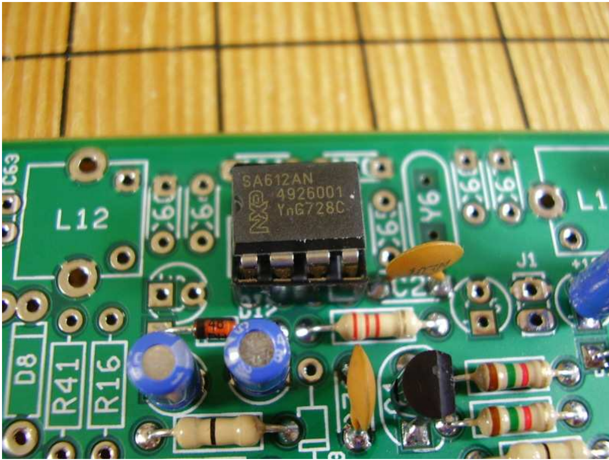
Figure 5.3: [3-1] U4 NE612 IC.
