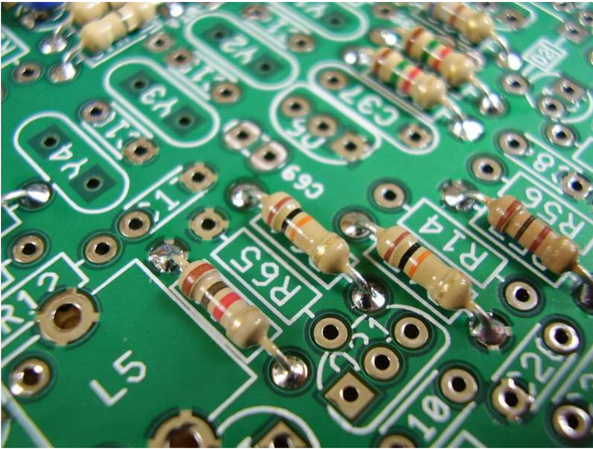
Figure 4.14: [2-16] R64 10K.
