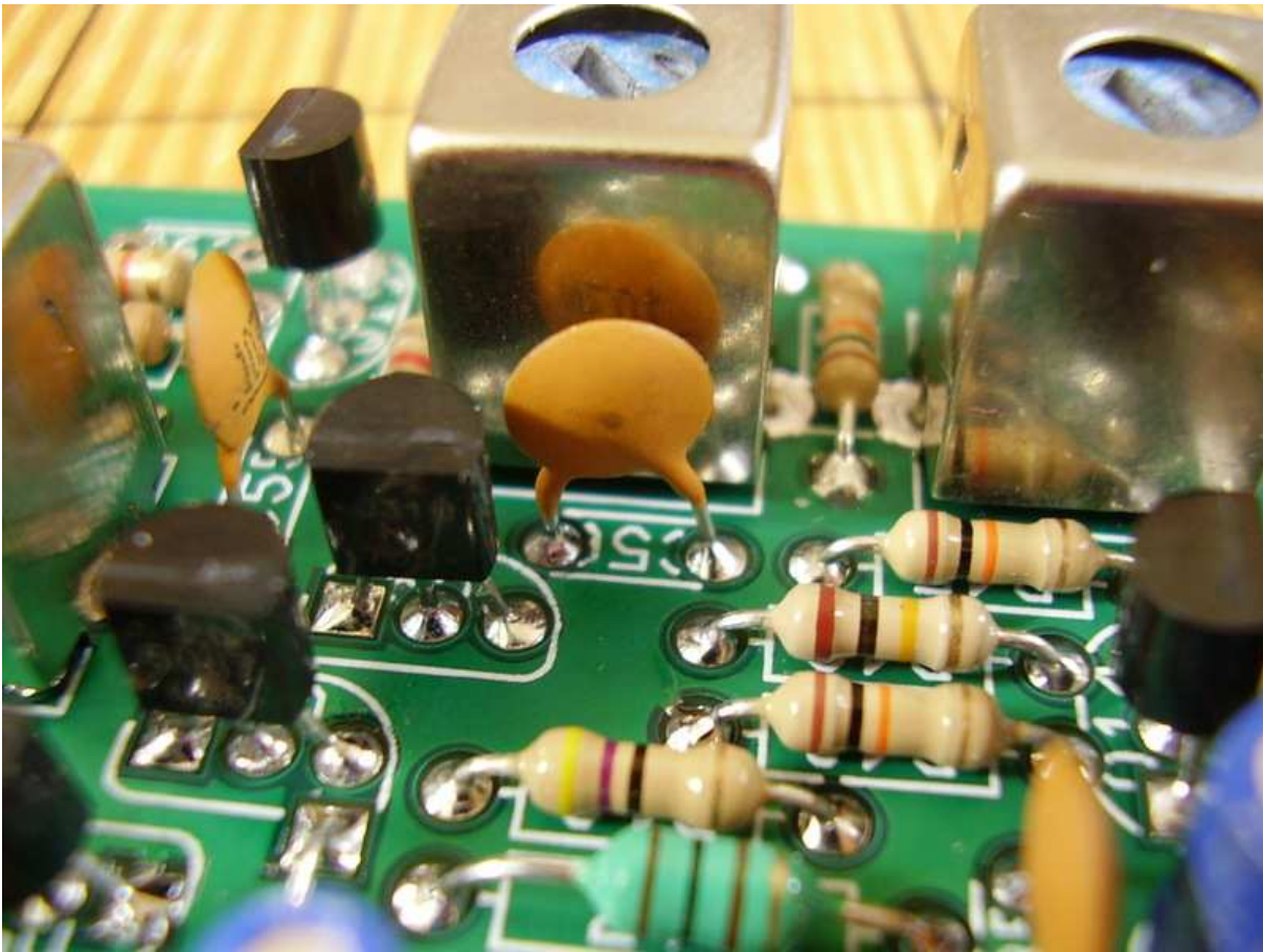
Figure 6.23: [4-21] C56 .01 \mu F.
