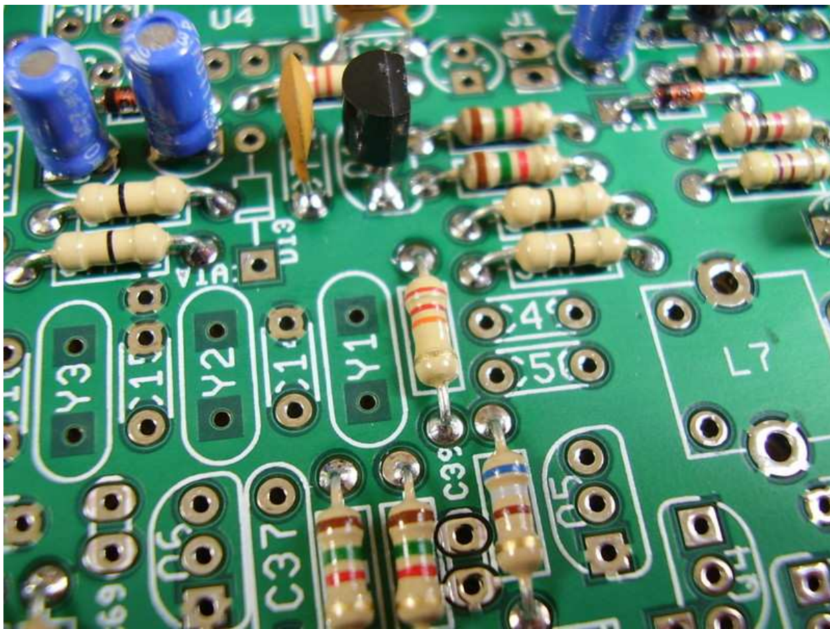
Figure 4.16: [2-18] R23 22K.
