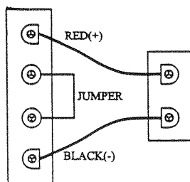
FIGURE 1-1. POWER SUPPLY ADAPTER CABLE (4 pin to 2 pin) View: Facing into plugs on cable ends
