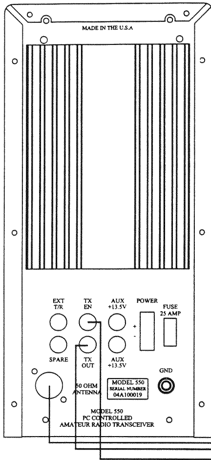
(REAR VIEW) Model 550 Pegasus
