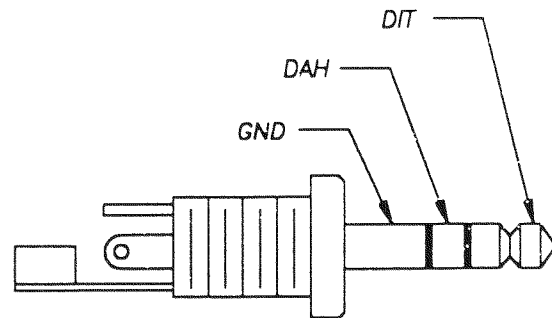
FIGURE 1-3 PADDLE WIRING FOR BUILT-IN ELECTRONIC KEYS
