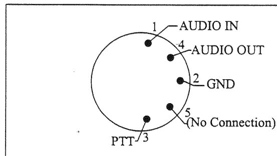
FIGURE 1-4 ACCESSORY JACK CONNECTIONS
