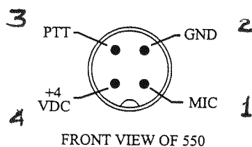
FIGURE 1-5 MICROPHONE CONNECTION
