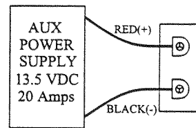
FIGURE 1-2. POWER SUPPLY CONNECTIONS (View from front of plug on end of cable)
