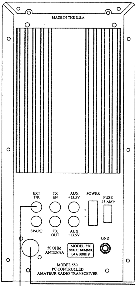
(REAR VIEW) Model 550 Pegasus
