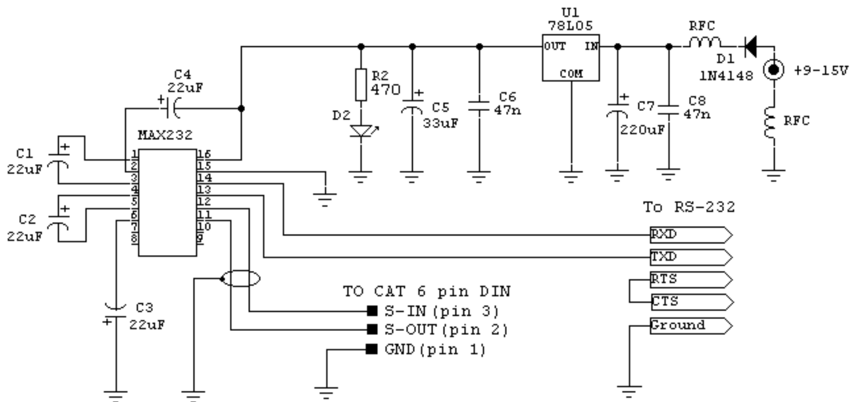
YAESU CAT INTERFACE (FIF-232 compatible)
