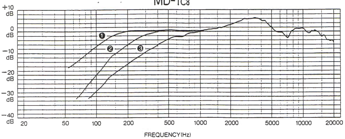
MD-1C8
