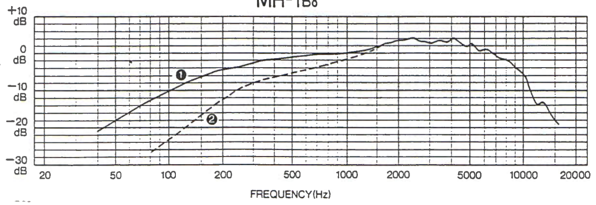
MH-1B8
