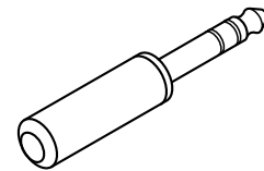
6.3 mm 3-contact Plug
