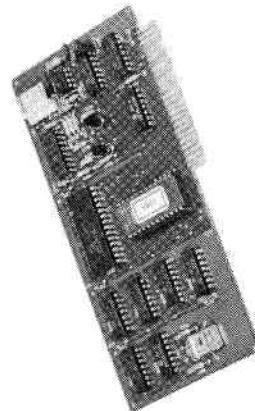
FIF-65A (for Apple II)
