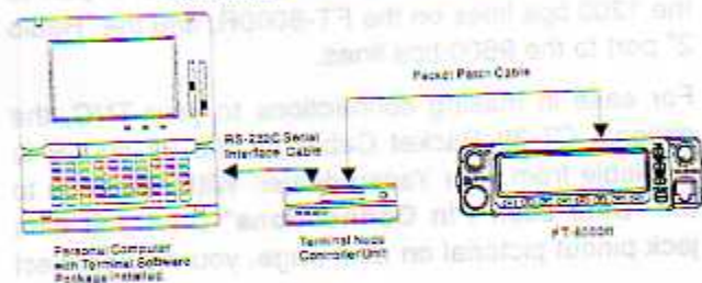
Station Interconnections for Digital Modes
