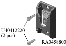
Front Panel Bracket
