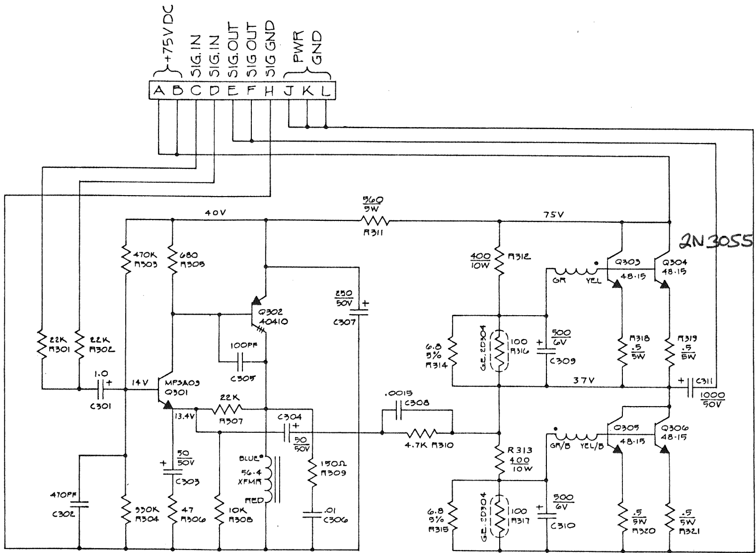
POWER MODULE (17-12)
