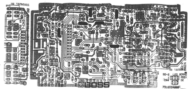
View from component side.
