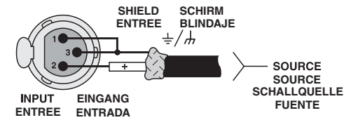
Figure 2.4 Unbalanced Input Connector Wiring
