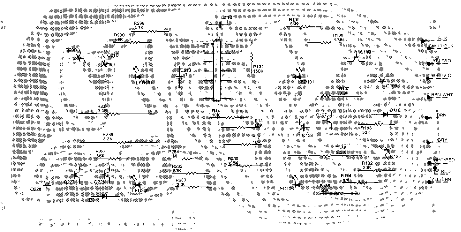
Fig. 6.8 PS-400 Display Module Foil Board Layout; P 9980B3
