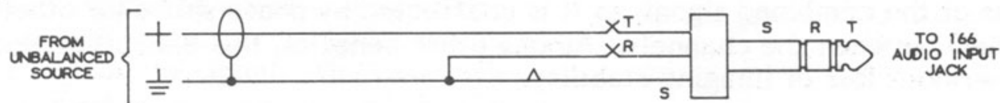
Figure 2a: Unbalanced sources, dual-conductor shielded cable
