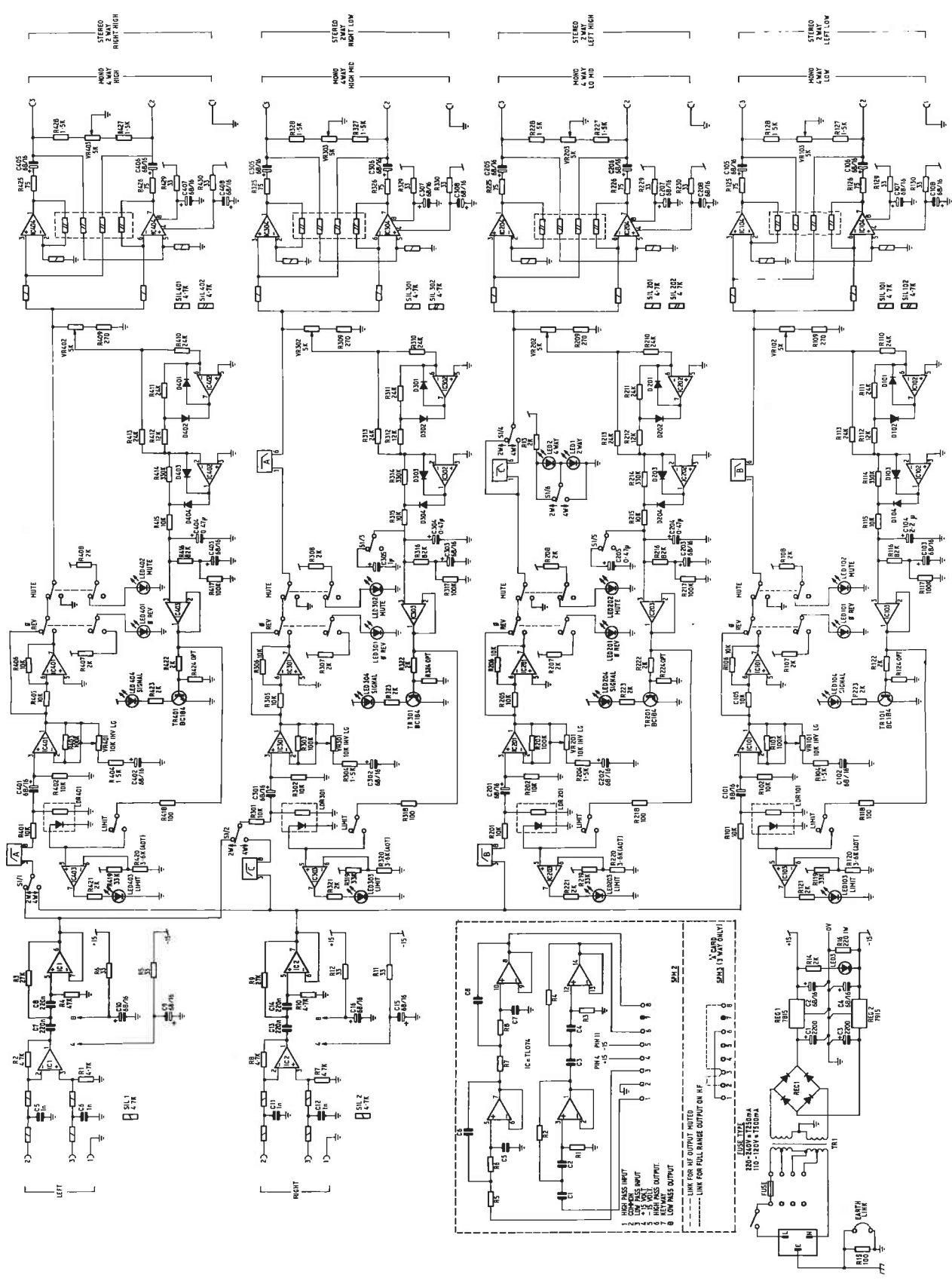
Fig 8.2 DD500 Circuit Diagram
