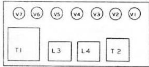
INSIDE VIEW OF AMPLIFIER
