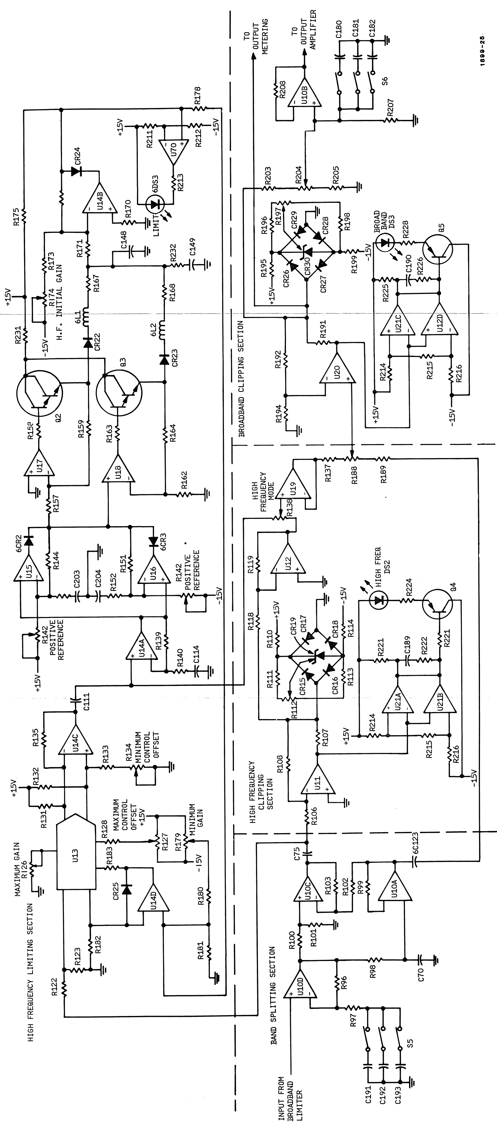
FIGURE 4-2. DETAILED BLOCK DIAGRAM FM LIMITER MODULE HIGH FREQUENCY PROTECTION SECTION
